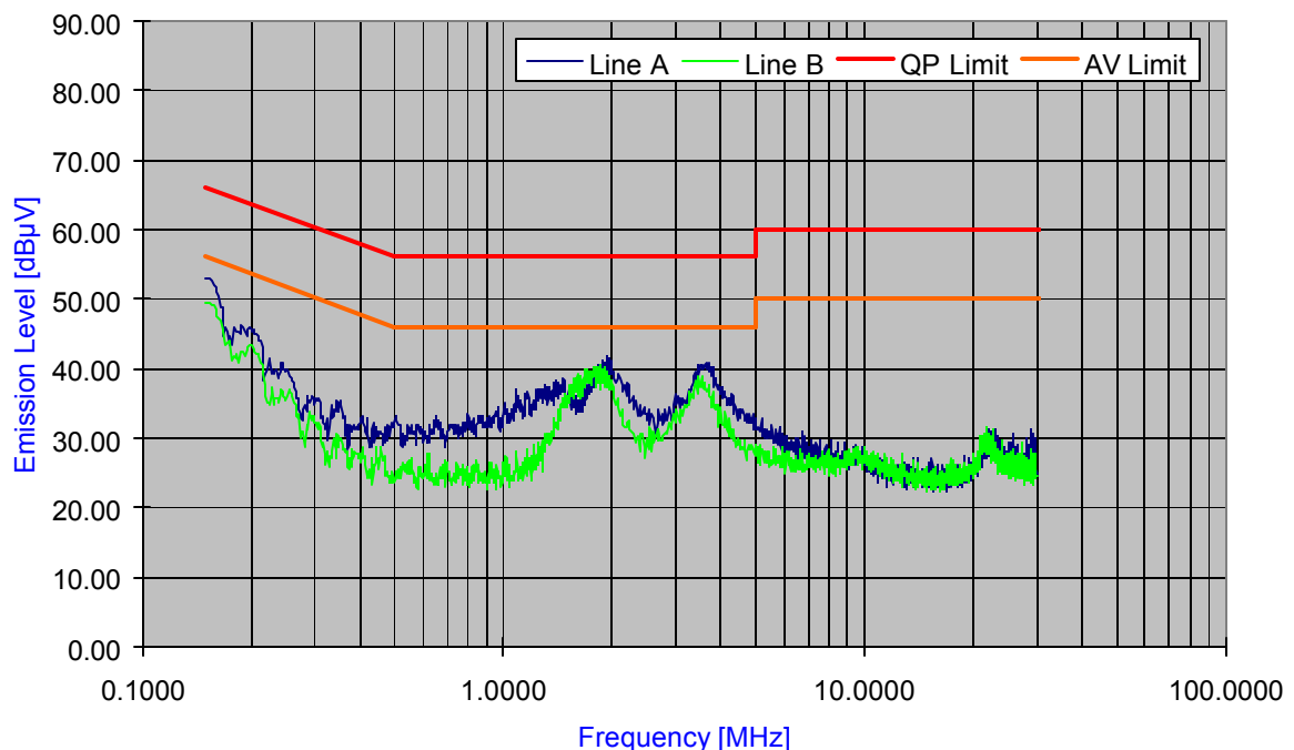
Plot 8-1. Line-Conducted Test Plot
