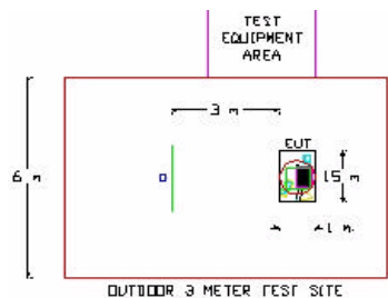
Figure 3-6. Dimensions of Outdoor Test Site
