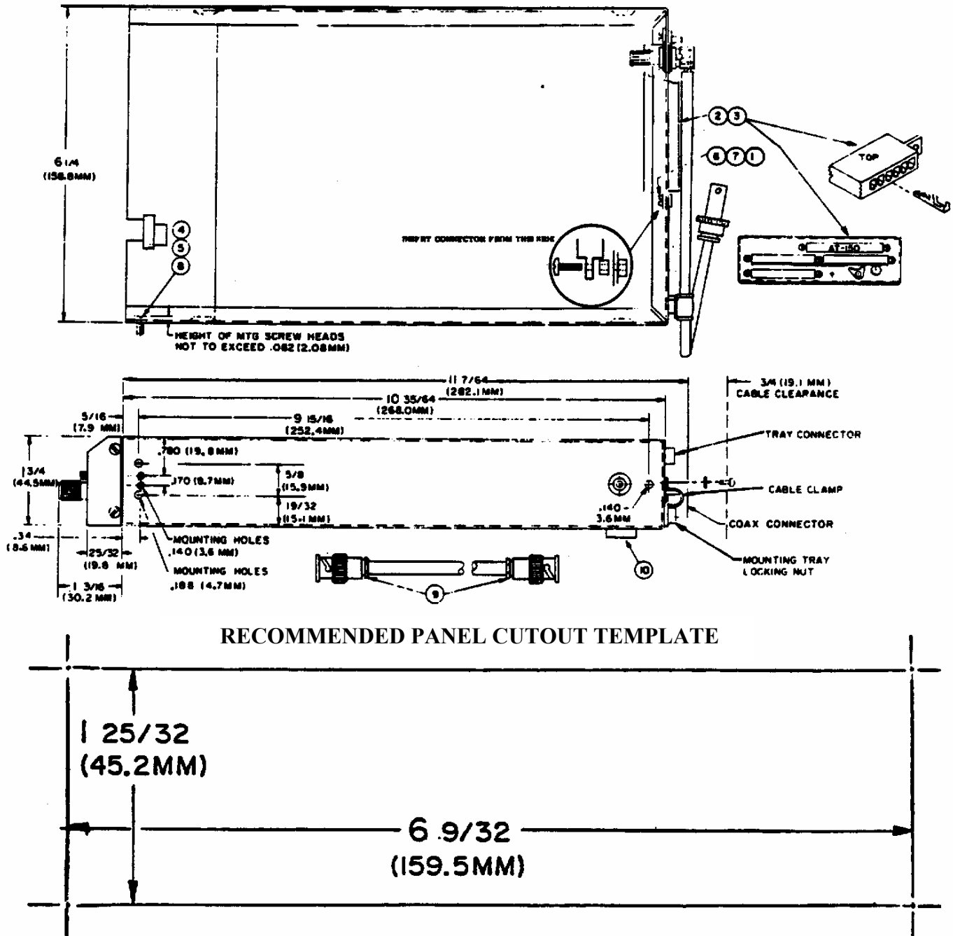
FIGURE 2-2. INSTALLATION DIAGRAM
