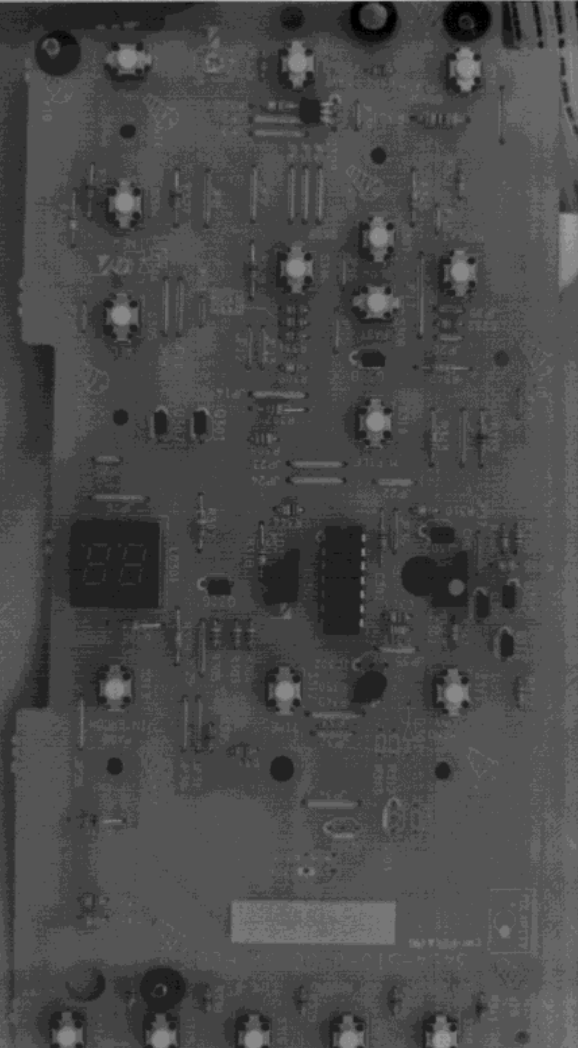
TOP VIEW OF TOP BASE BOARD WITHOUT ENCLOSURE FCC ID: AAL-TC-925
