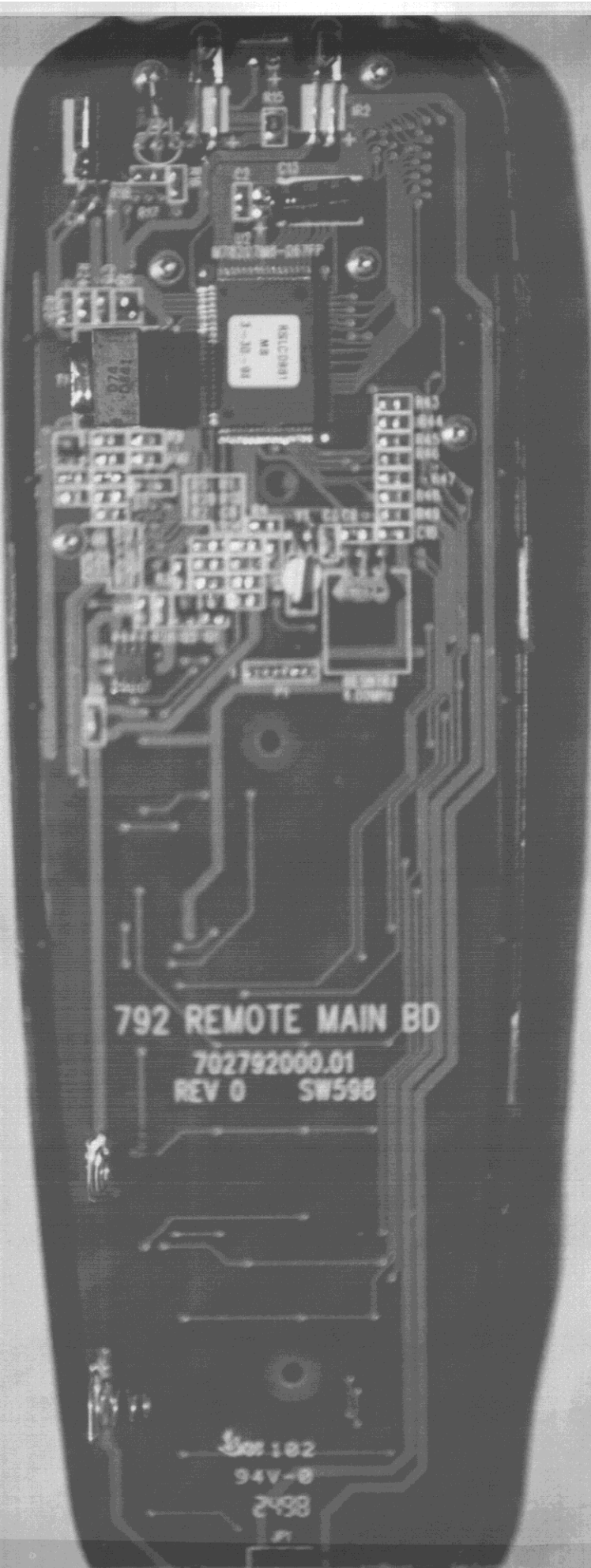
TOP VIEW OF MAIN PCB BOARD WITHOUT RF PUCK FCC ID: AAO1501935
