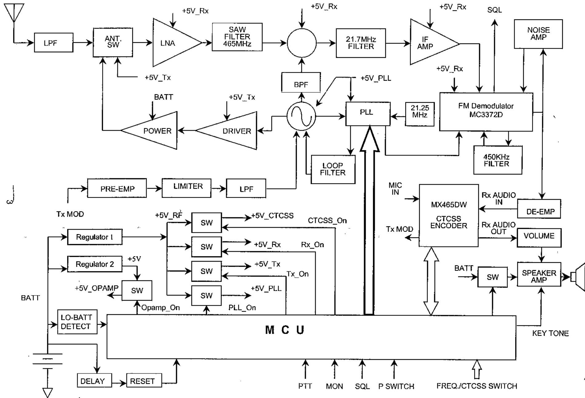
BLOCK DIAGRAM
