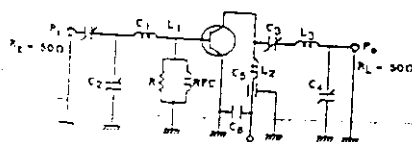
FIG. 1. TEST CIRCUIT
