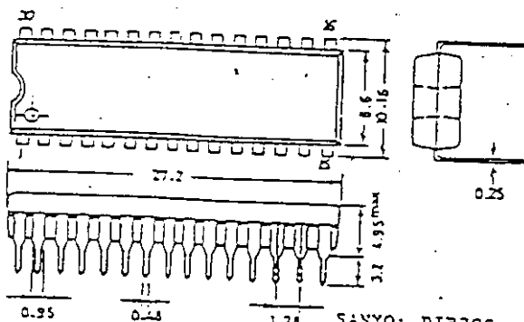
Case Outline 3061-D30SNC (unit:mm)
