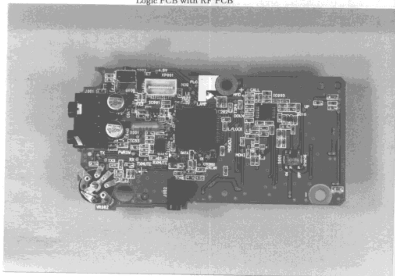
Logic PCB CPU side with Shield Cover
