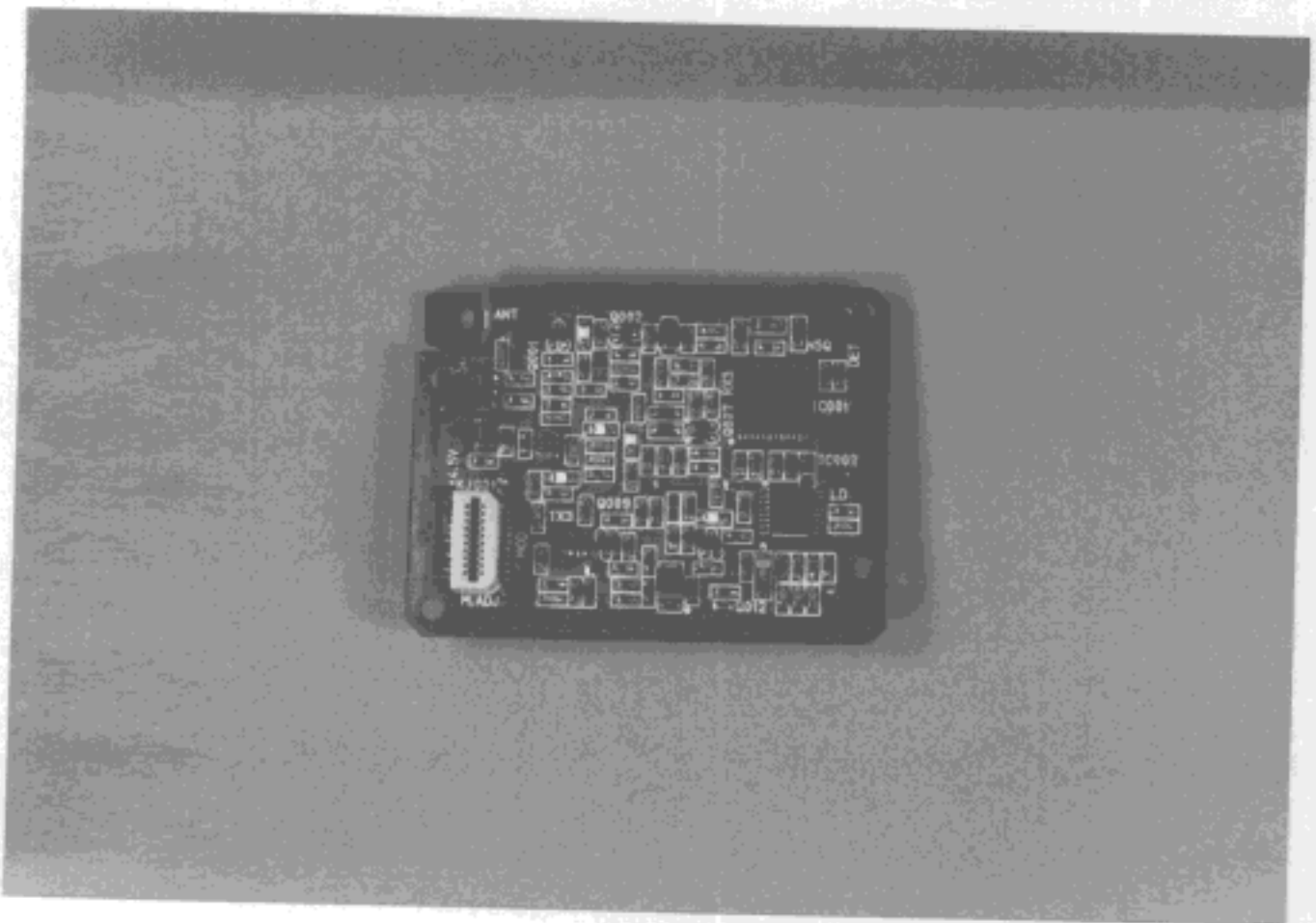
RF PCB Connector side without Shield Case
