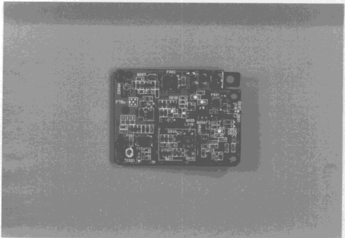
RF PCB VCO side without Shield Case
