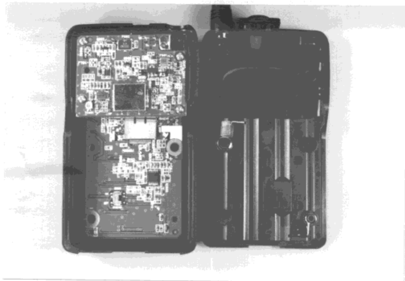
Transceiver Unit without Rear Case
