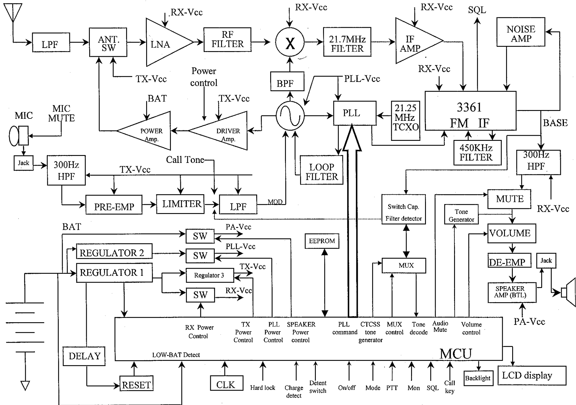
21-1813 14-channel FRS radio block diagram
