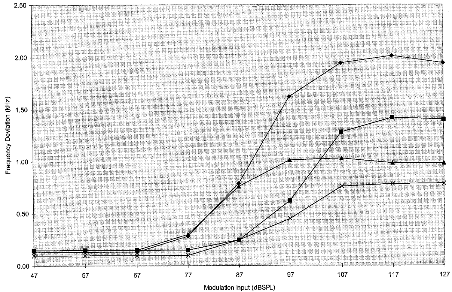
Modulation Limiting Characteristic
