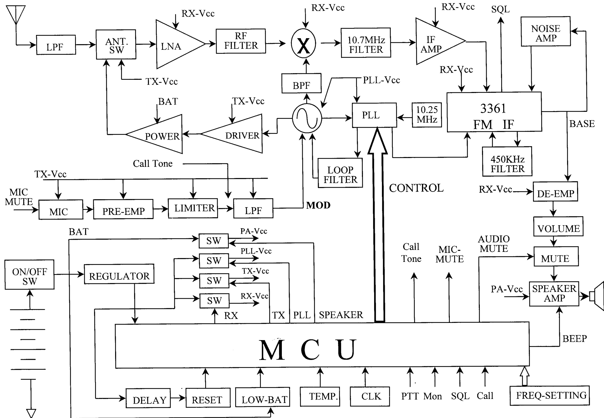
21-1820 2-channel FRS radio block diagram
