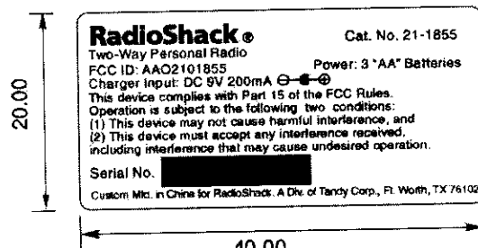
RATING LABEL Scale 1:1
