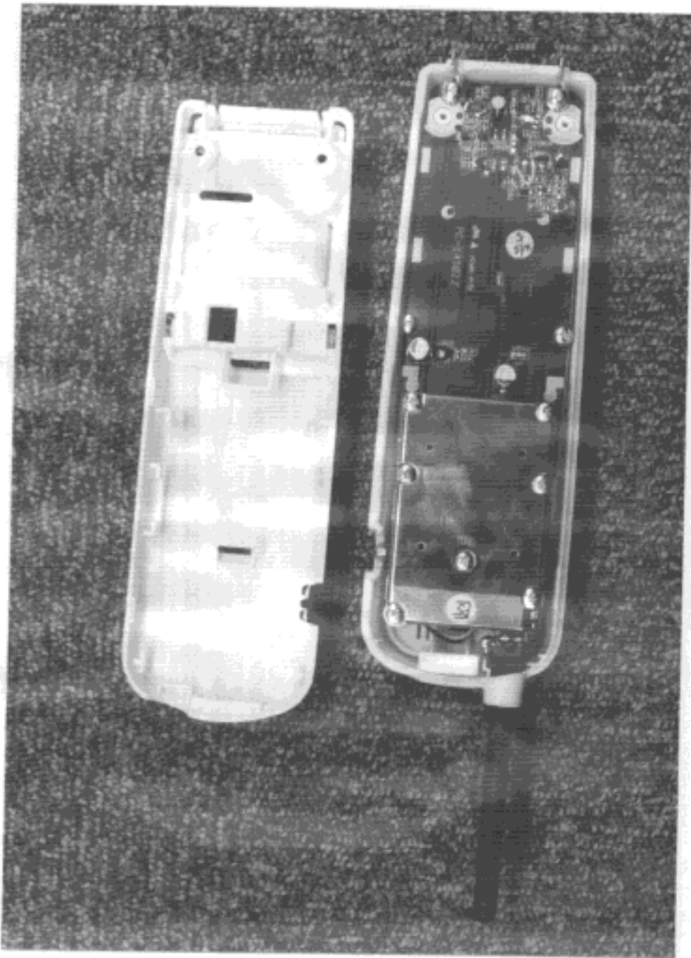
Internal view of the handset Rear cover removed
