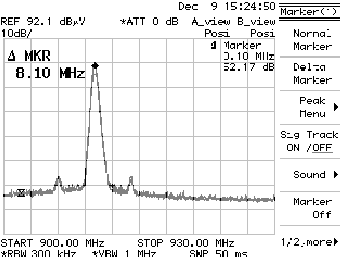
Fig 1, Trace A without modulation, Trace B with 1kHz Modulation.
