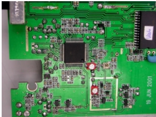
Internal Photo - 2
