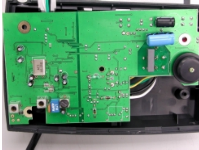
Internal Photo - 3
