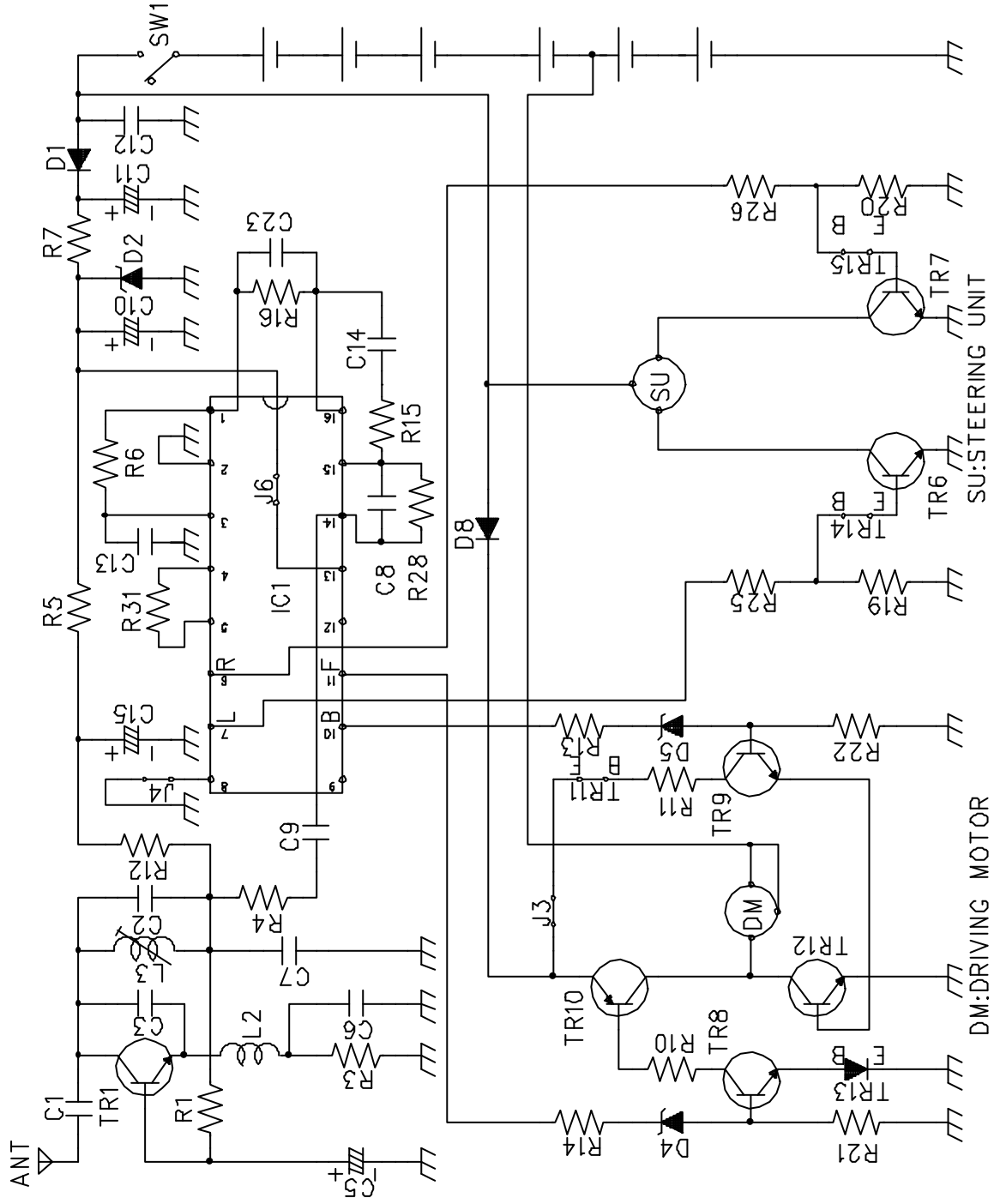
NO.RP7300CR CIRCUIT DIAGRAM 2000.12.8 MM.
