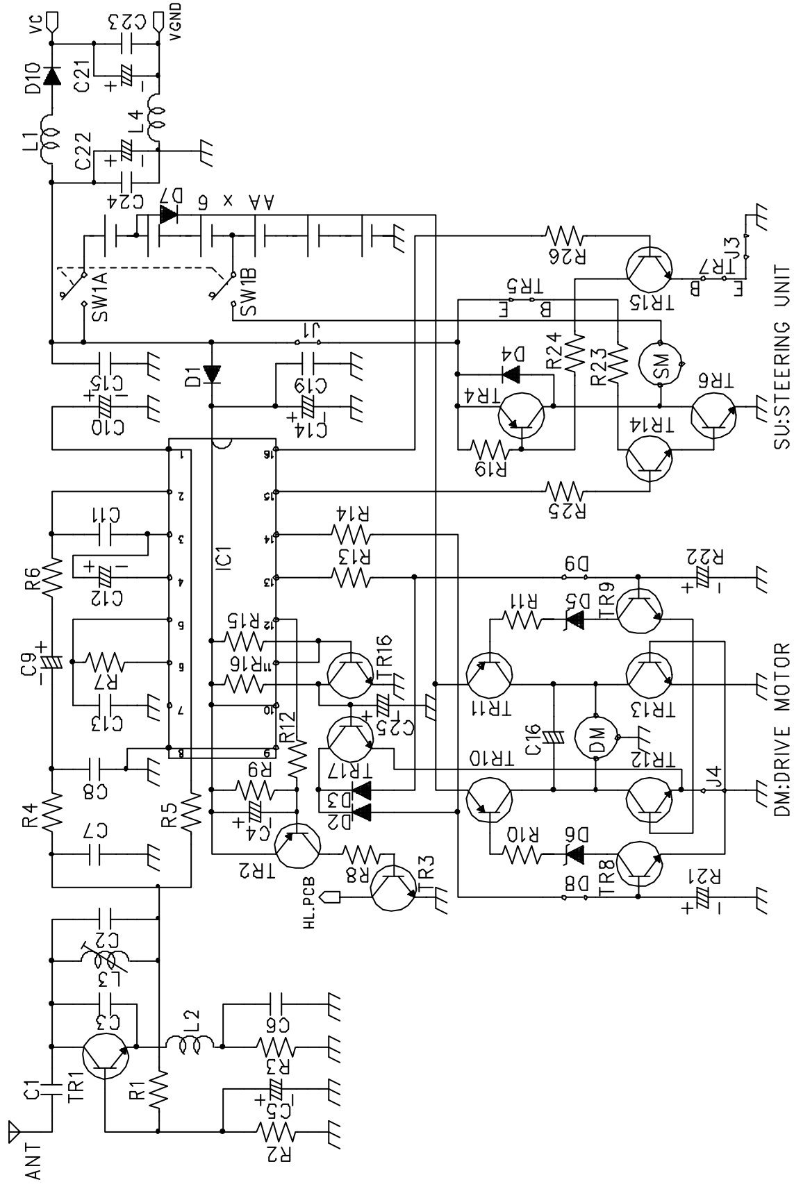
NO.RN6330 CIRCUIT DIAGRAM
