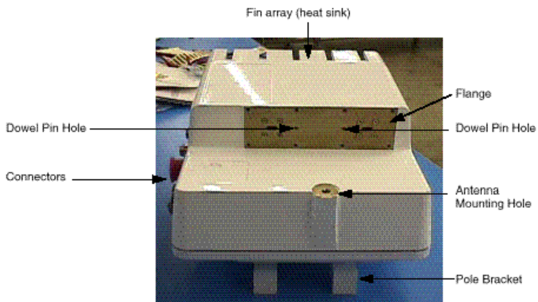
Figure 3 - Antenna Placement on the BTR2400
