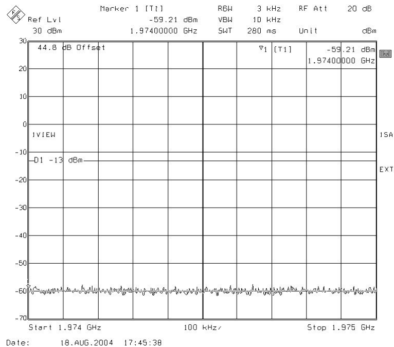
Figure 17: 1974 MHz – 1975 MHz Out-of-block emissions (Channel 810, Pmax), GMSK modulation ( BTS18000 )
