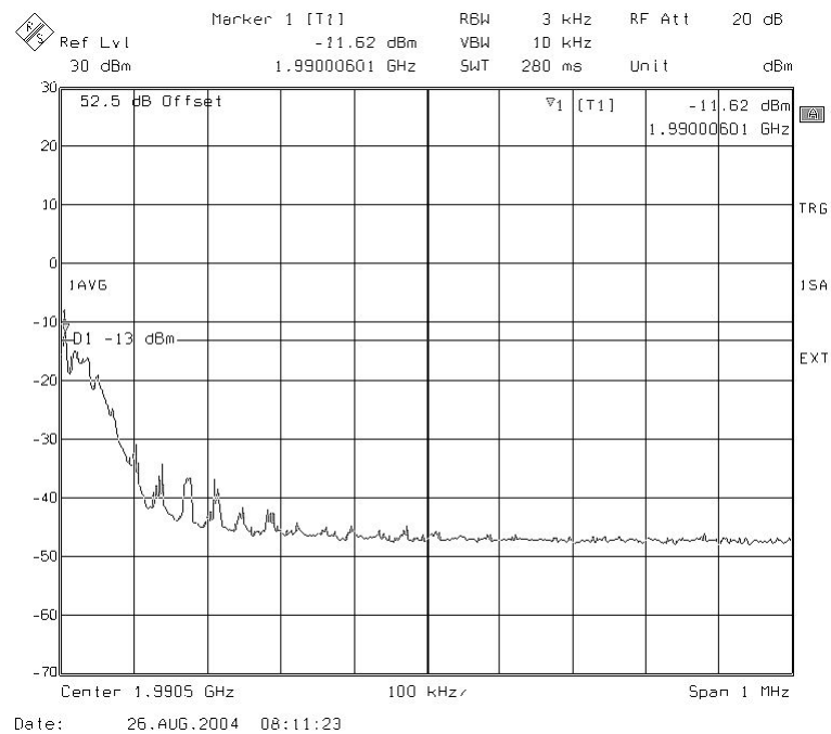
Figure 29 : +1 MHz adjacent band (Channel 810, Pmax), 8PSK modulation (GSM 18000 BTS + MCPA PWW BTS)
