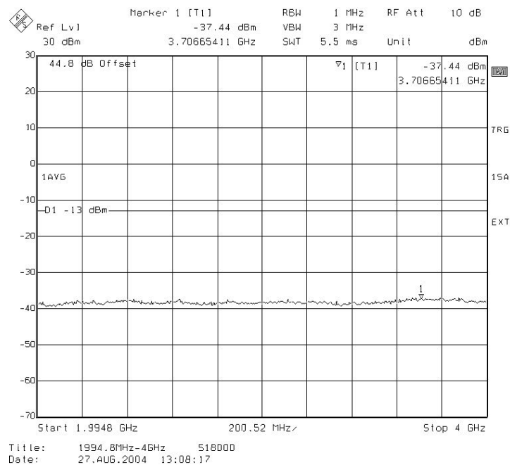
Figure 19: 1994 MHz –4 GHz Out-of-block emissions (Channel 810, Pmax), GMSK modulation (BTS18000)
