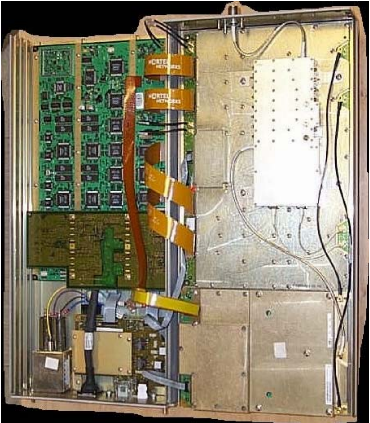
E-Cell – Radio Section Internal View
