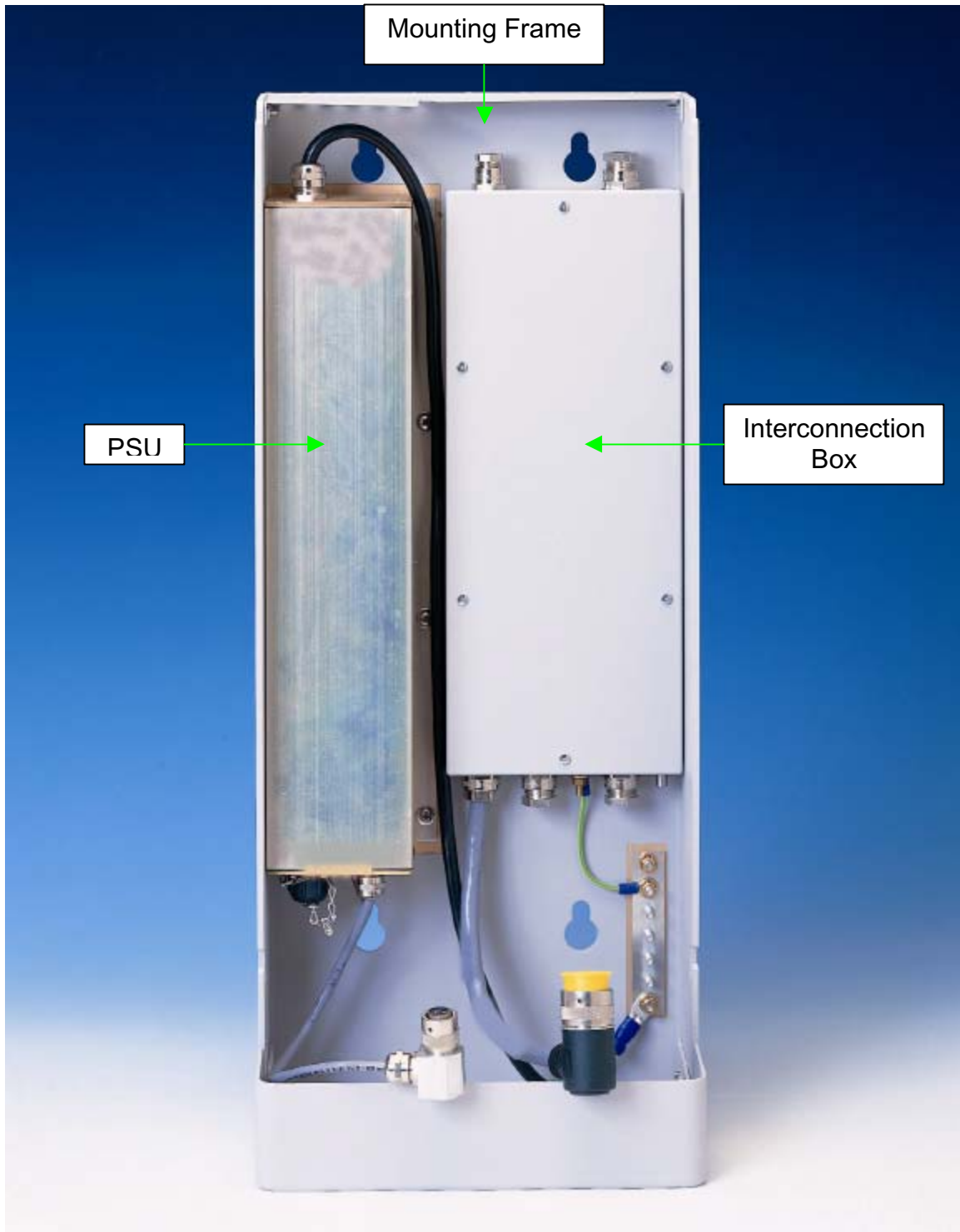
E-Cell – Installation Kit with the PSU Option
