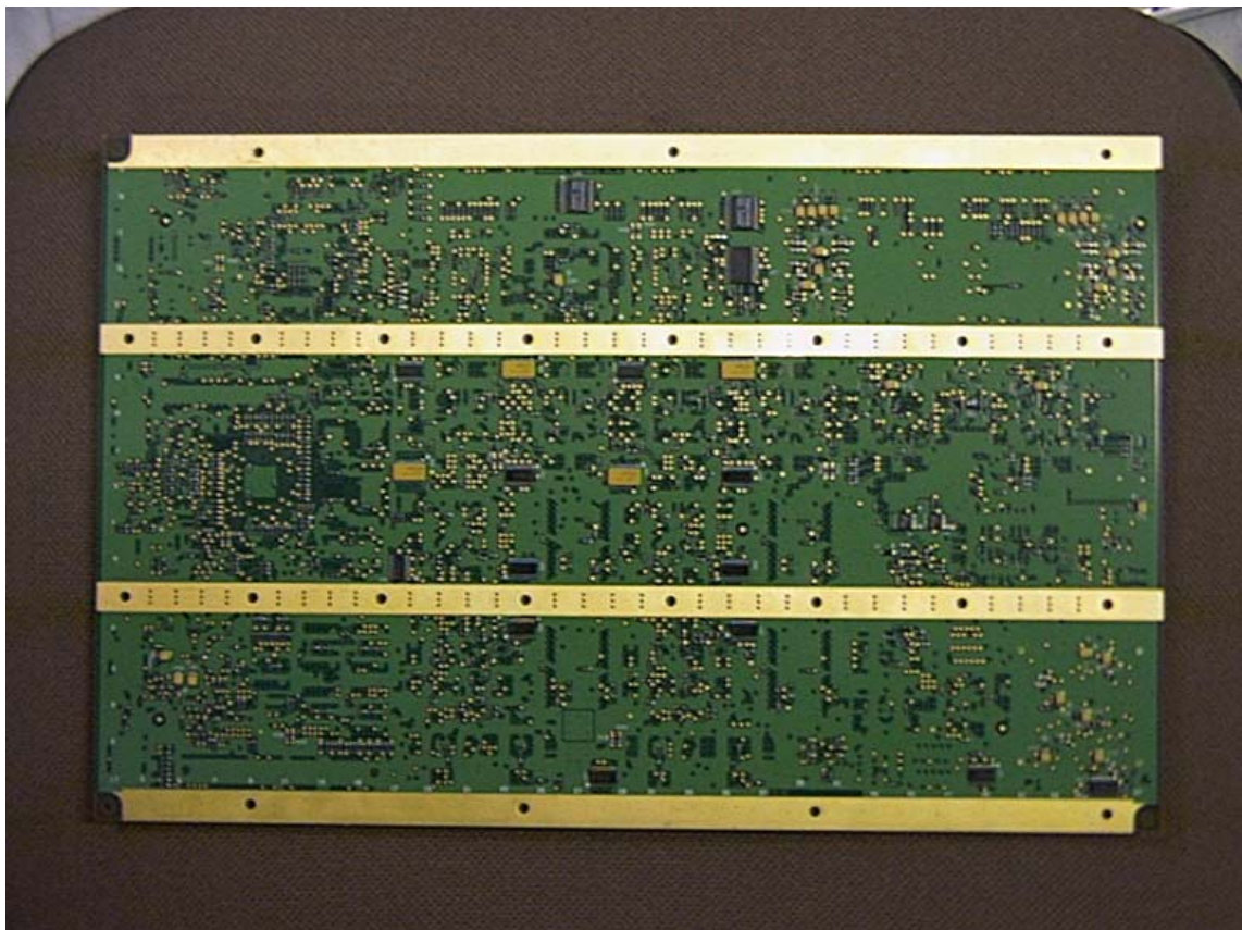
Figure 4: Logic board (Bottom view)
