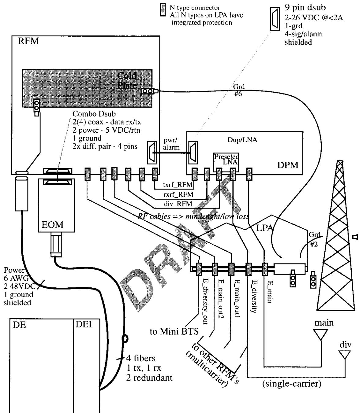
Figure 1 RFMA Interconnect
