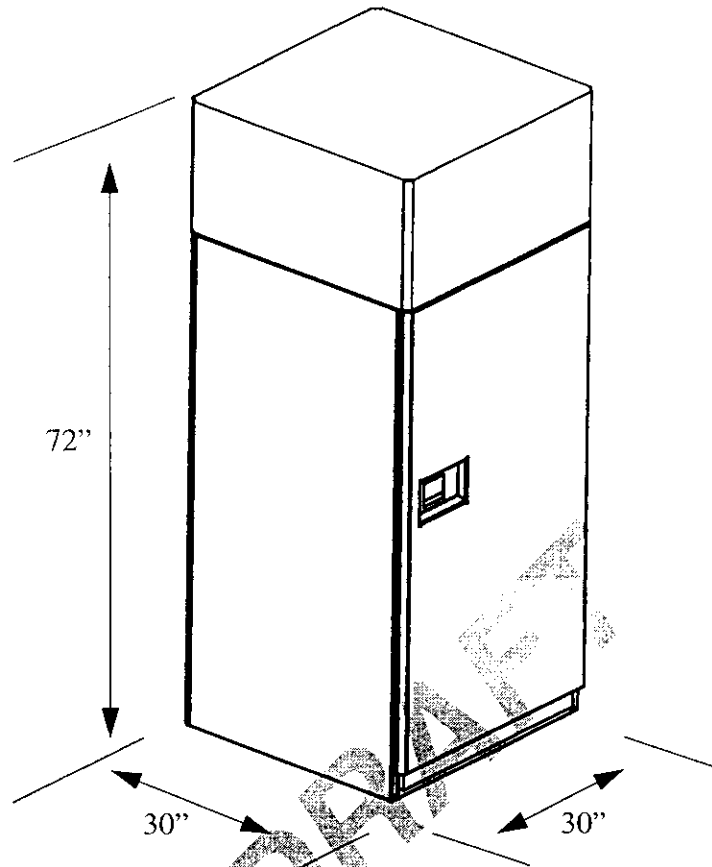
ISOMETRIC VIEW
