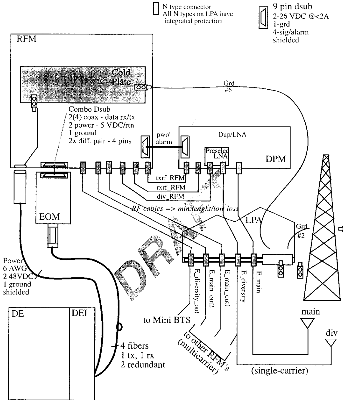
Figure 1 RFMA Interconnect
