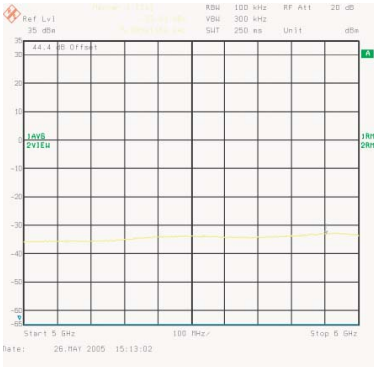
Figure 13 : Conducted Spurious Emissions - Channel 308 (5 GHz - 6 GHz)
