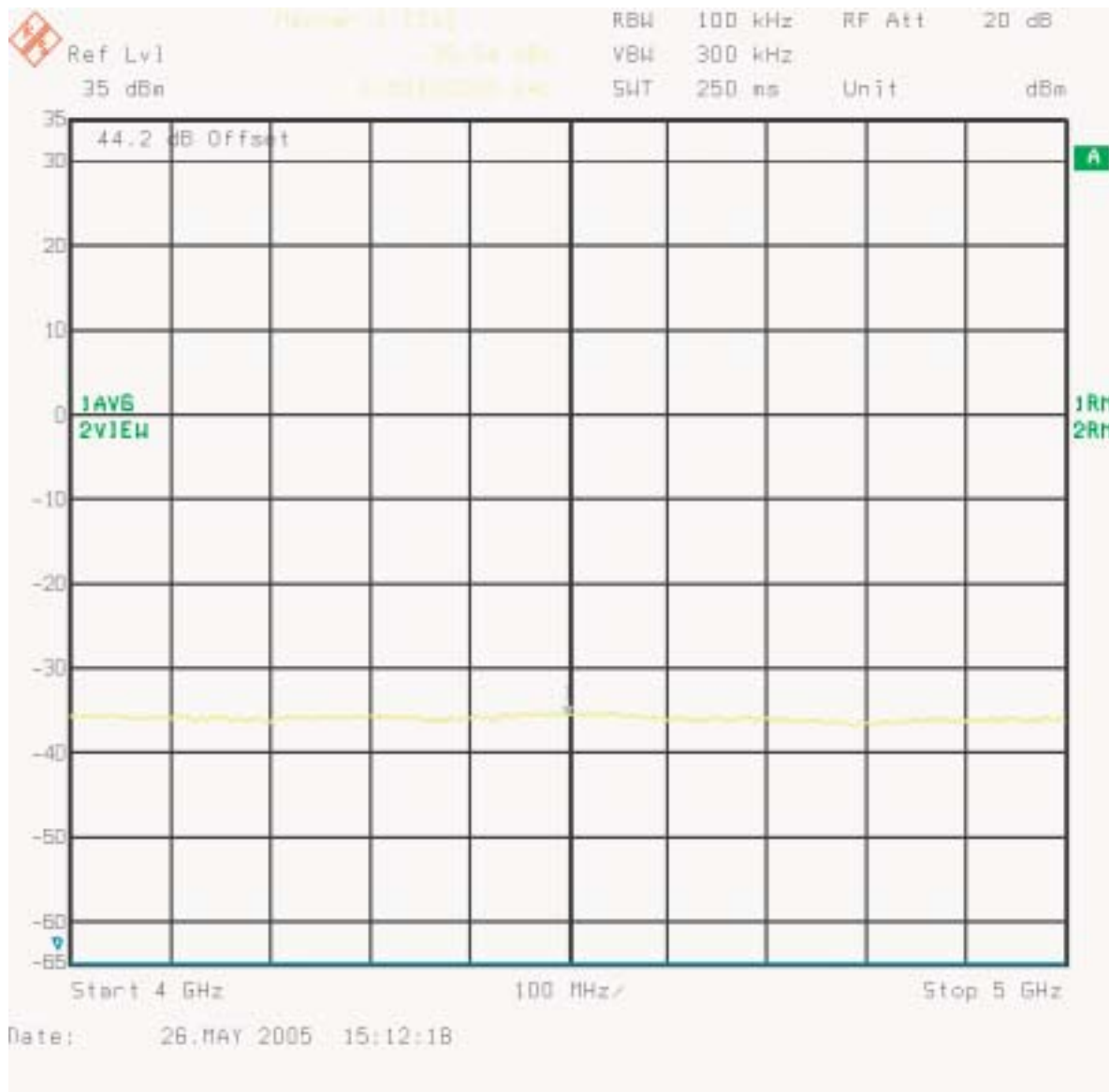
Figure 12 : Conducted Spurious Emissions - Channel 308 (4 GHz - 5 GHz)
