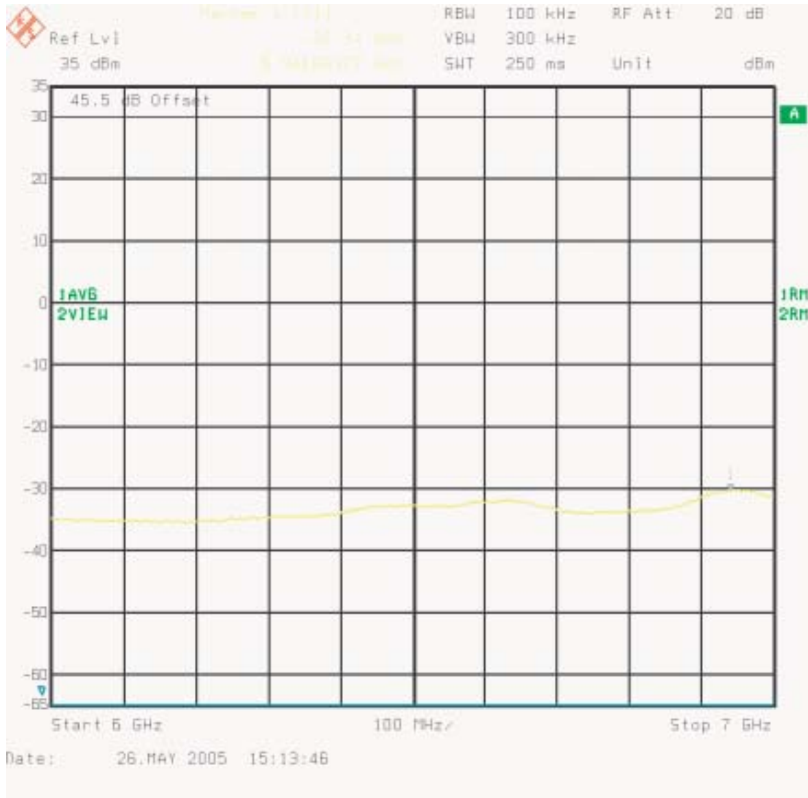
Figure 14 : Conducted Spurious Emissions - Channel 308 (6 GHz - 7 GHz)
