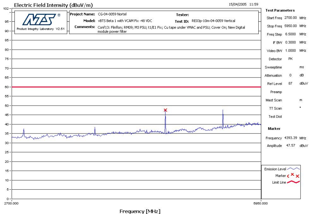
Figure 8 RE - Vertical - 2.7 GHz - 5.95 GHz Pre-Scan
