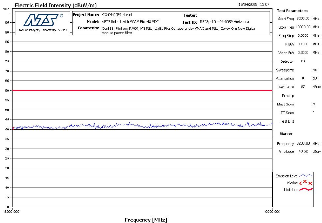
Figure 11 RE - Horizontal - 8.2 GHz - 10 GHz Pre-scan
