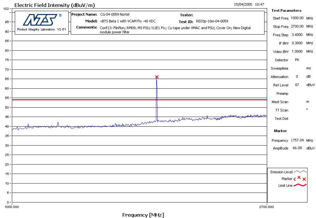
Figure 5 RE - Horizontal - 1 GHz - 2.7 GHz Pre-scan
