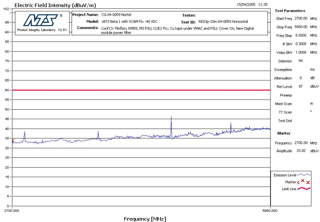
Figure 7 RE - Horizontal - 2.7 GHz - 5.95 GHz Pre-scan
