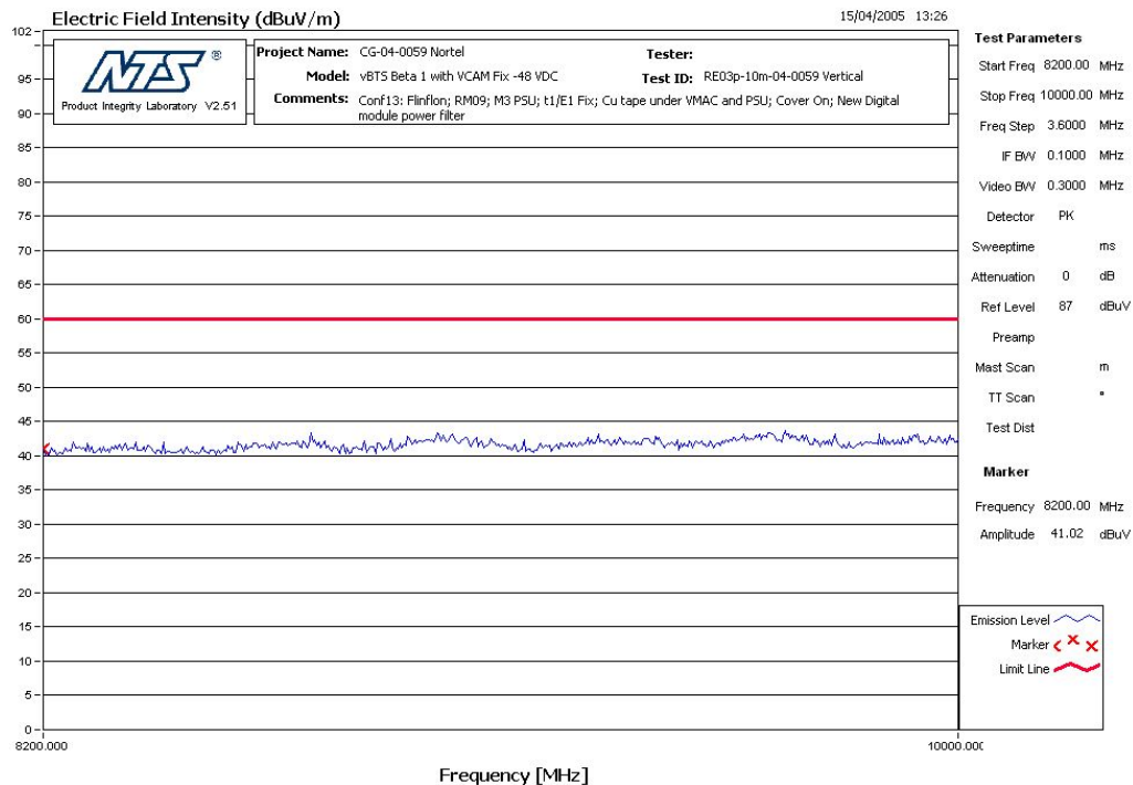
Figure 12 RE - Vertical - 8.2 GHz - 10 GHz Pre-Scan
