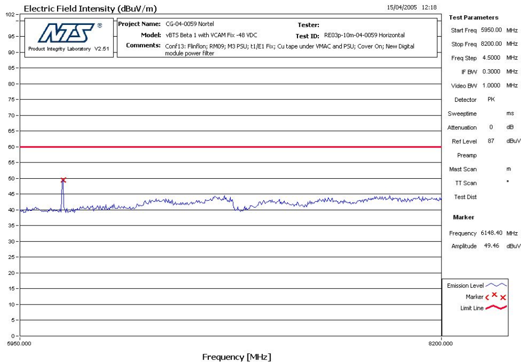
Figure 9 RE - Horizontal - 5.95 GHz - 8.2 GHz Pre-scan
