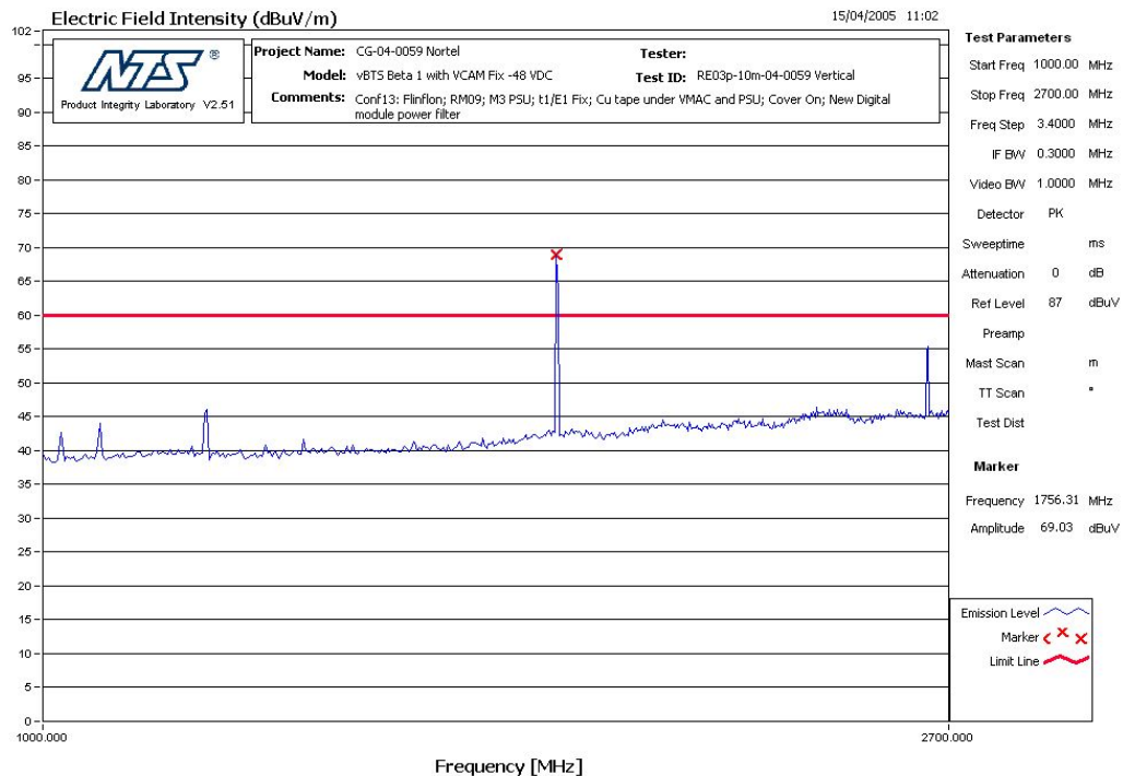
Figure 6 RE - Vertical - 1 GHz - 2.7 GHz Pre-Scan
