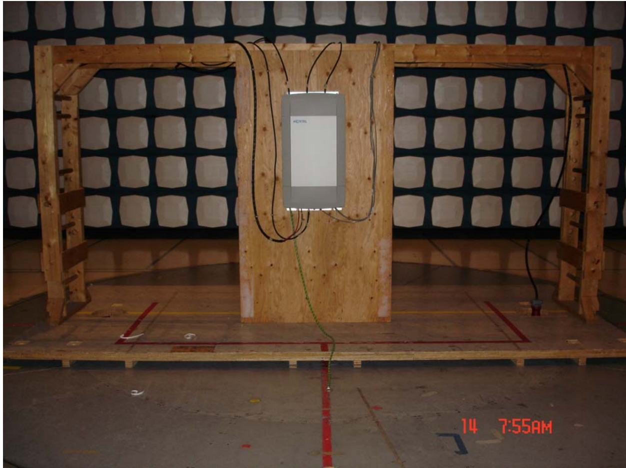
Figure 4 RE 30 MHz - 10 GHz EUT Configuration
