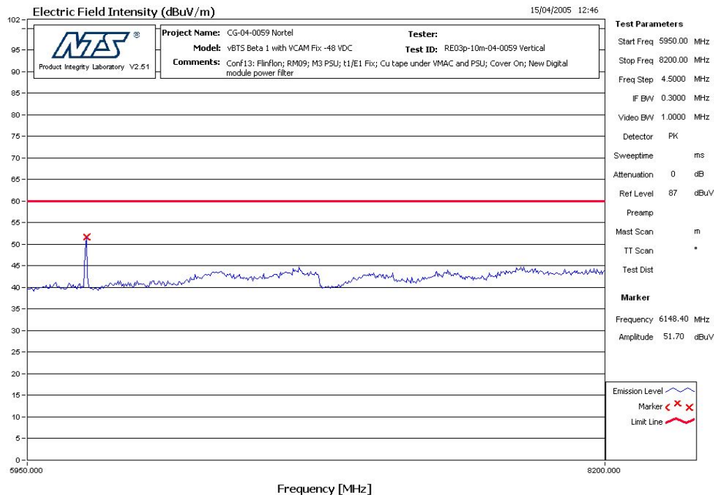
Figure 10 RE - Vertical - 5.95 GHz - 8.2 GHz Pre-Scan
