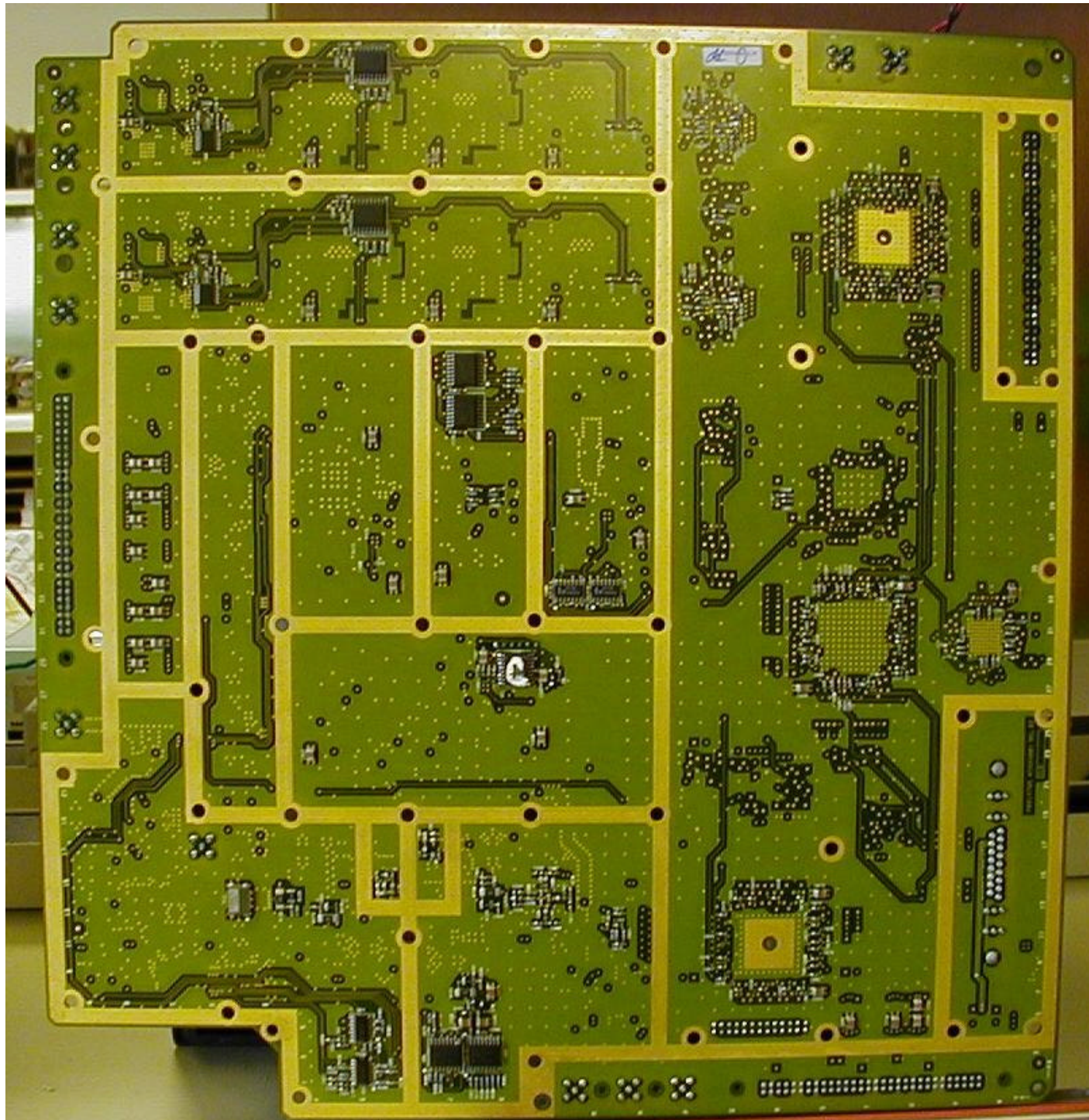
TRM-2000 [800 MHz] Internal Photo 1
