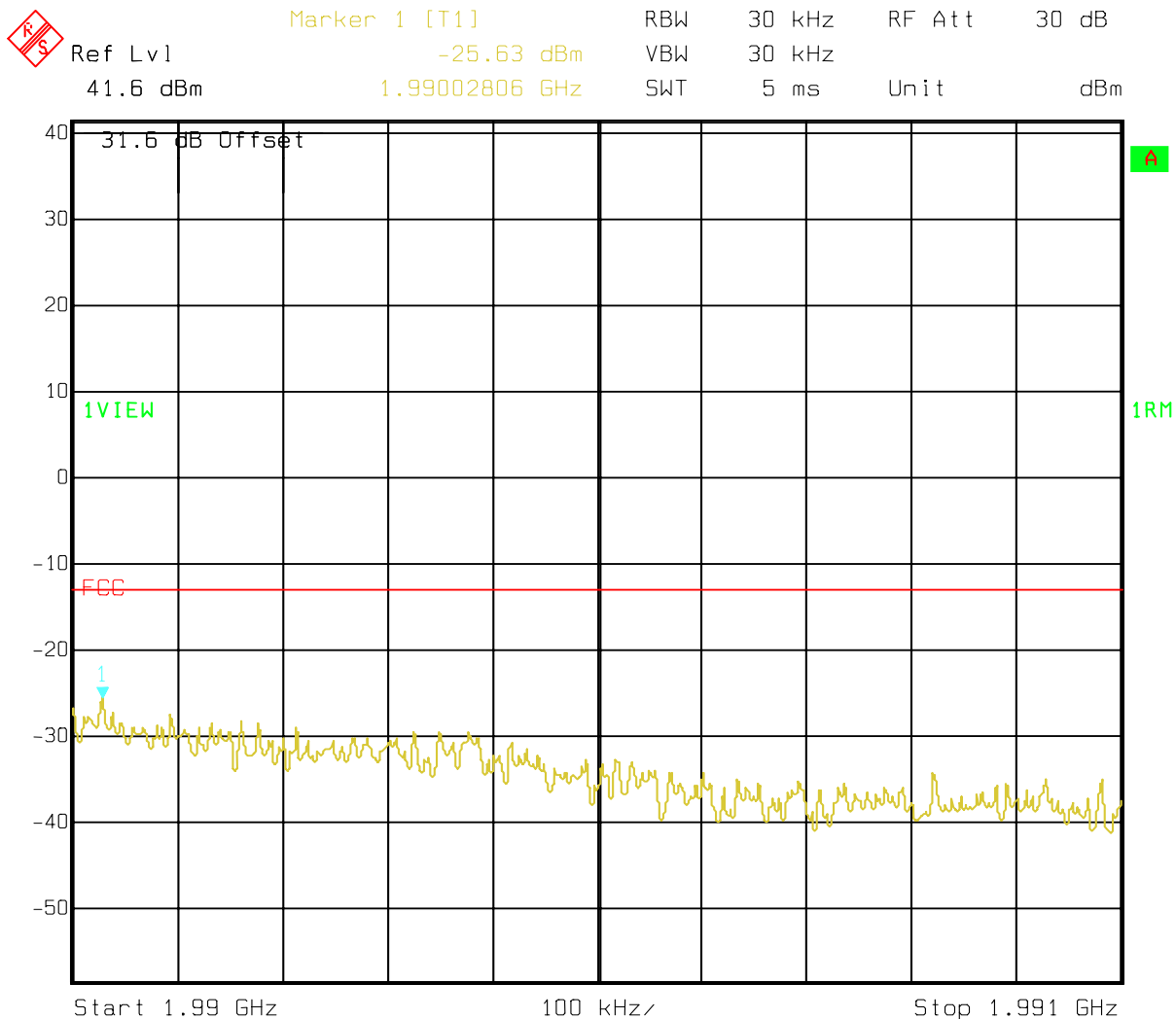
Figure 9 : Conducted Spurious Emissions - DPM, Channel 1175 (Adjacent 1 Mhz)
