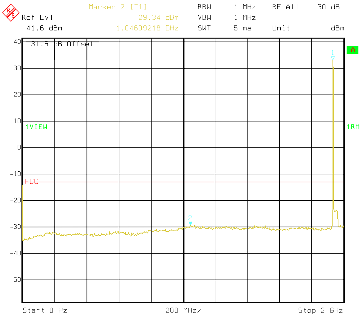
Figure 10 : Conducted Spurious Emissions - DPM, Channel 25 (10 kHz - 2 GHz)
