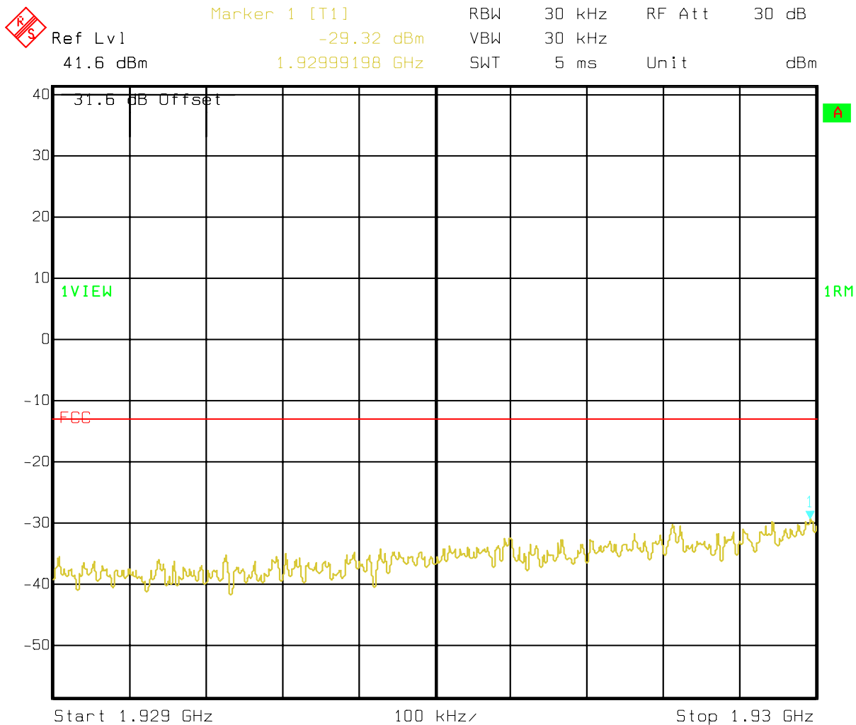
Figure 7 : Conducted Spurious Emissions - Triplexer, Channel 25 (Adjacent 1 Mhz)
