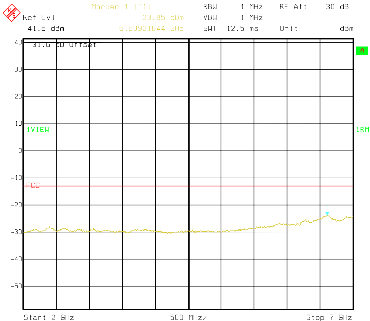
Figure 12 : Conducted Spurious Emissions - DPM, Channel 25 (2 GHz - 7 GHz)
