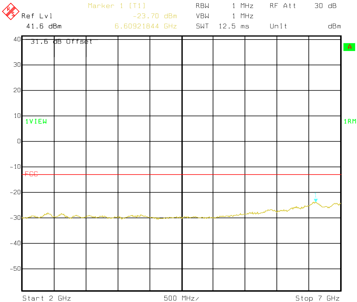
Figure 13 : Conducted Spurious Emissions - Triplexer, Channel 25 (2 GHz - 7 GHz)
