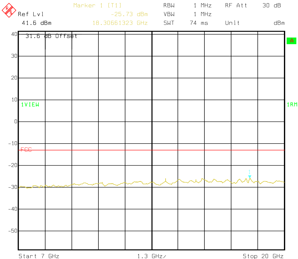
Figure 14 : Conducted Spurious Emissions - DPM, Channel 25 (7 GHz - 20 GHz)
