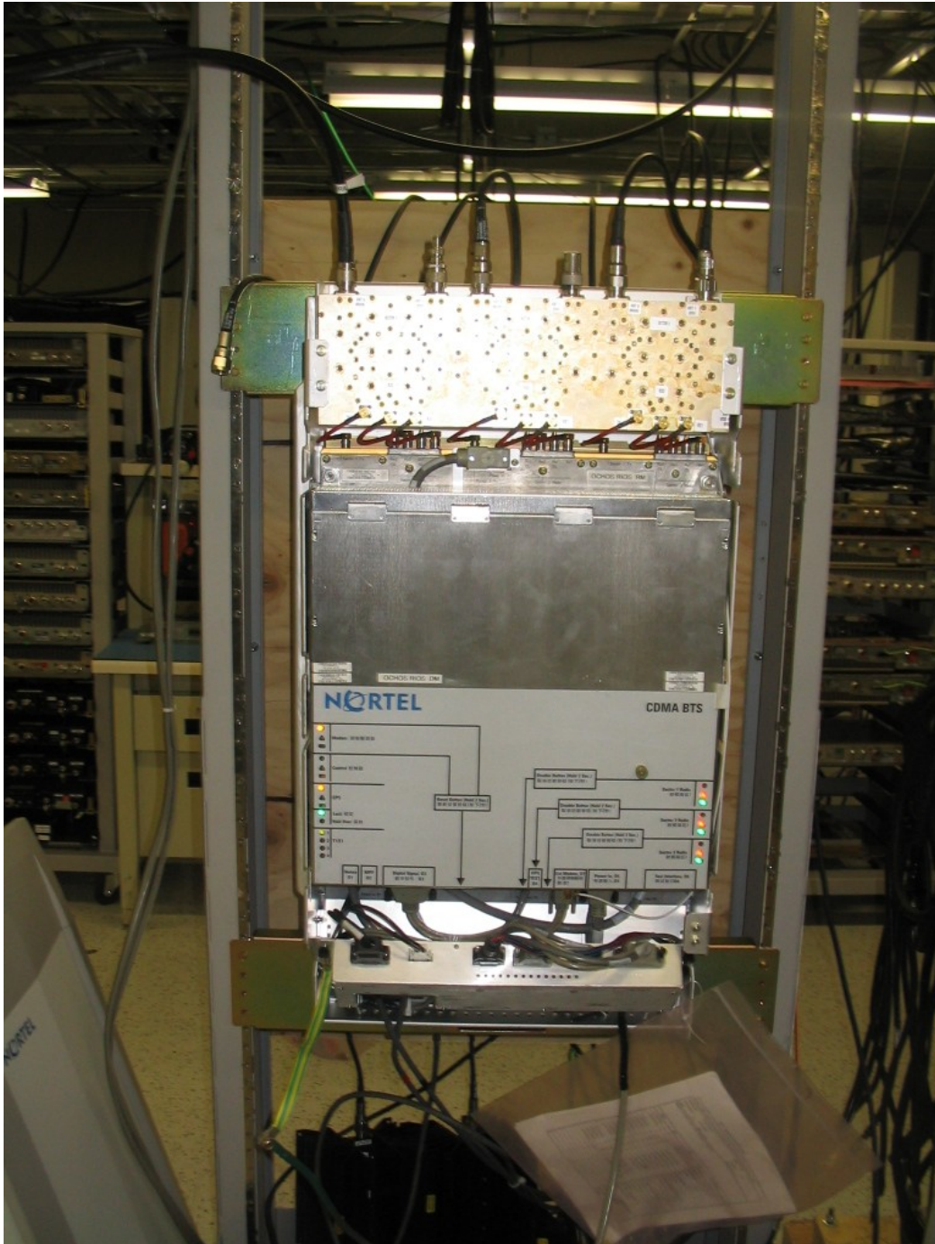
Nortel Networks vBTS 3030 Front View With Cover OFF
