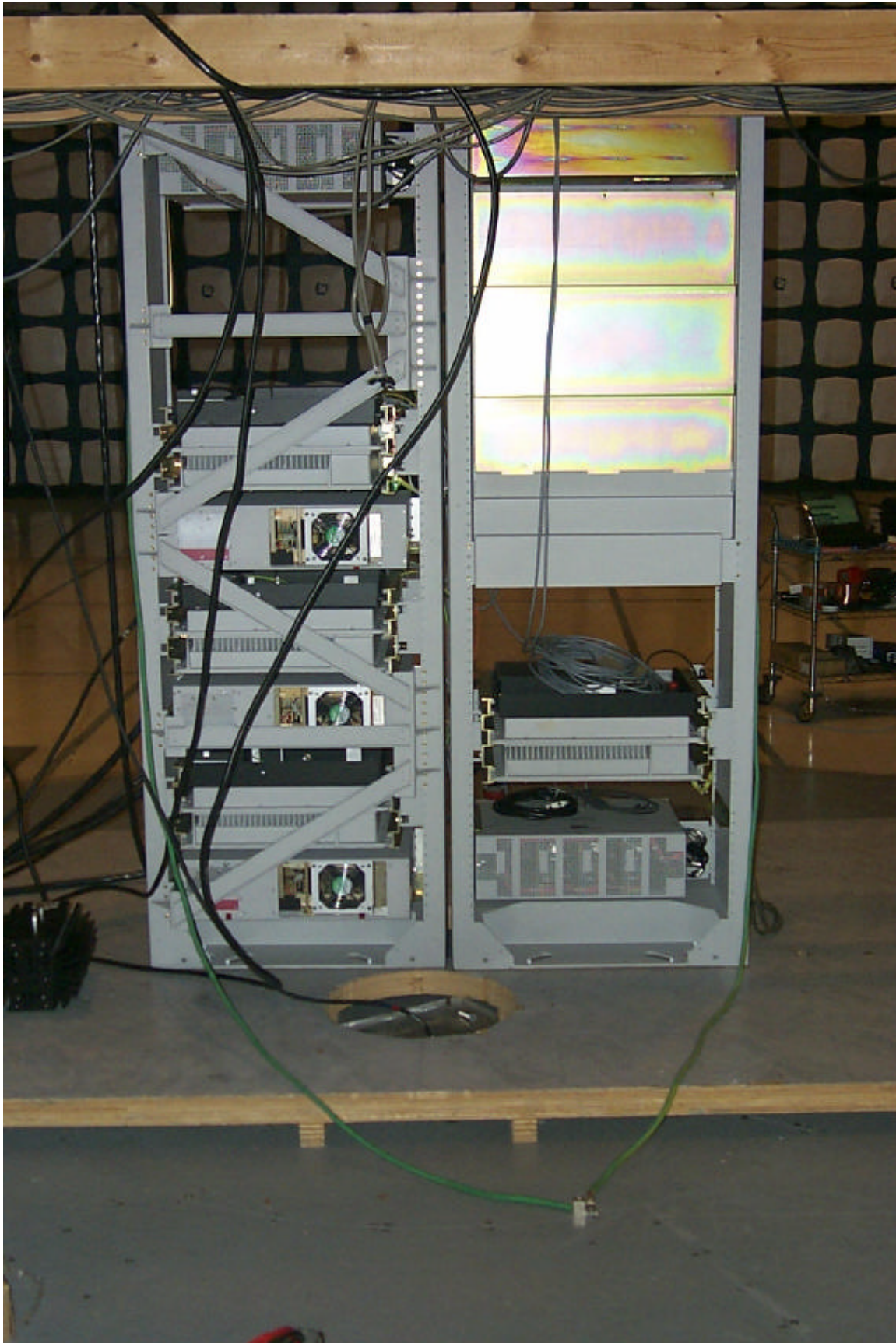
Nortel 800 MHz Flexible Radio Module AB6NT800EFRM Rural Cell with EFRMS rear view
