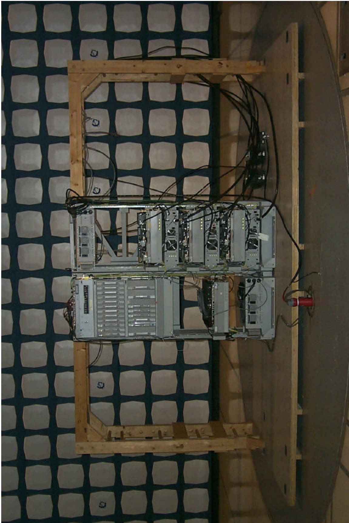
Nortel 800 MHz Flexible Radio Module AB6NT800EFRM Rural Cell system Radiated emissions setup (Front view)
