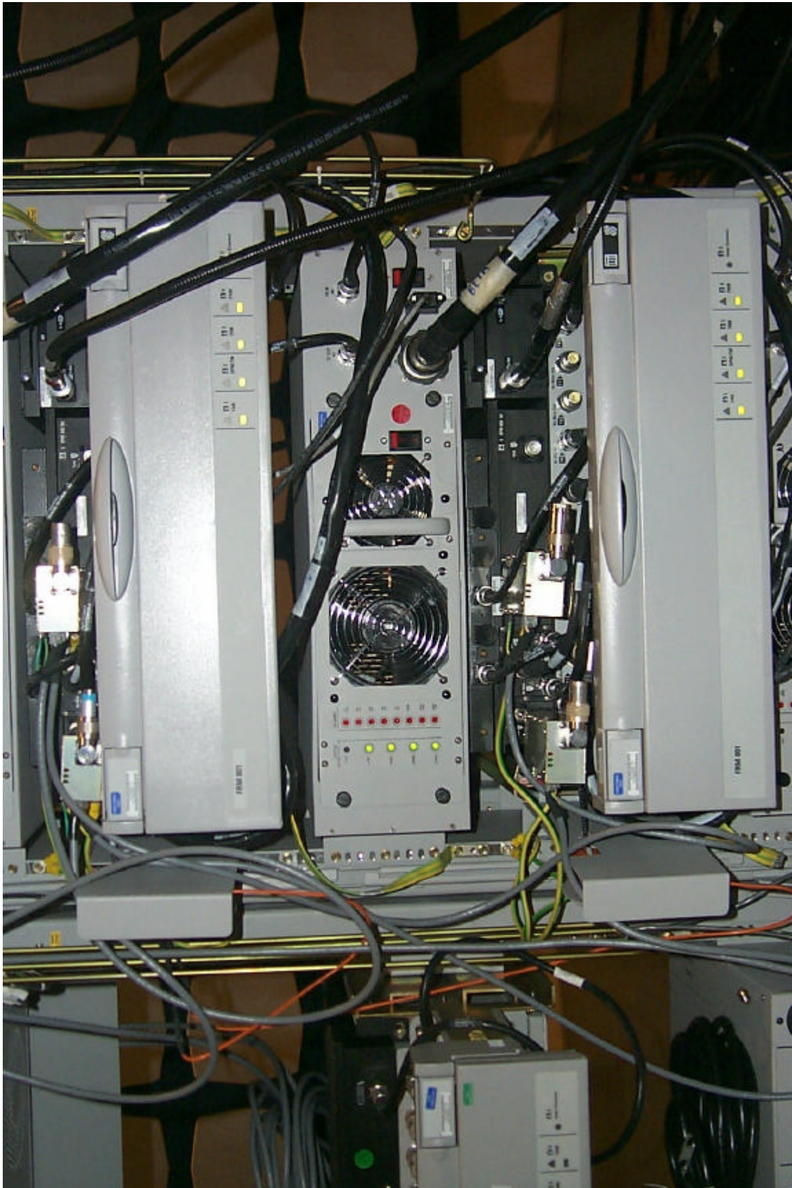
Nortel 800 MHz Flexible Radio Module AB6NT800EFRM EFRM Front view
