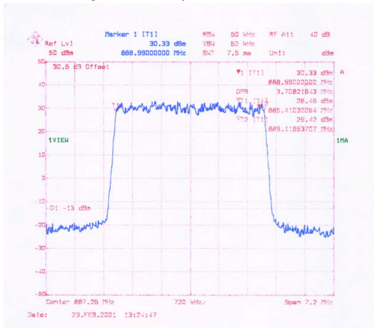
Figure 4: Plot of Occupied Bandwidth: 3 Carrier
