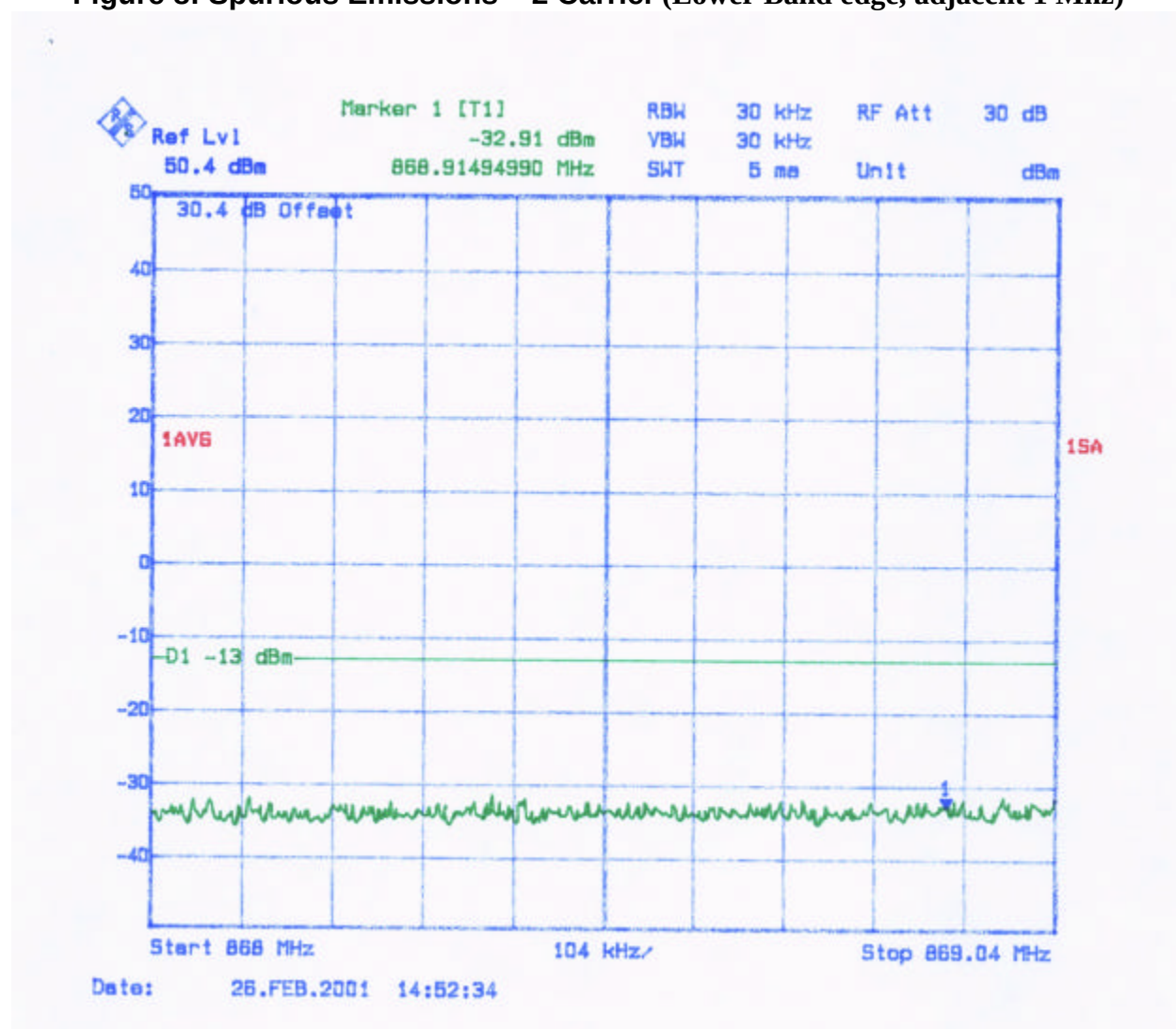
Figure 8: Spurious Emissions – 2 Carrier (Lower Band edge, adjacent 1 Mhz)
