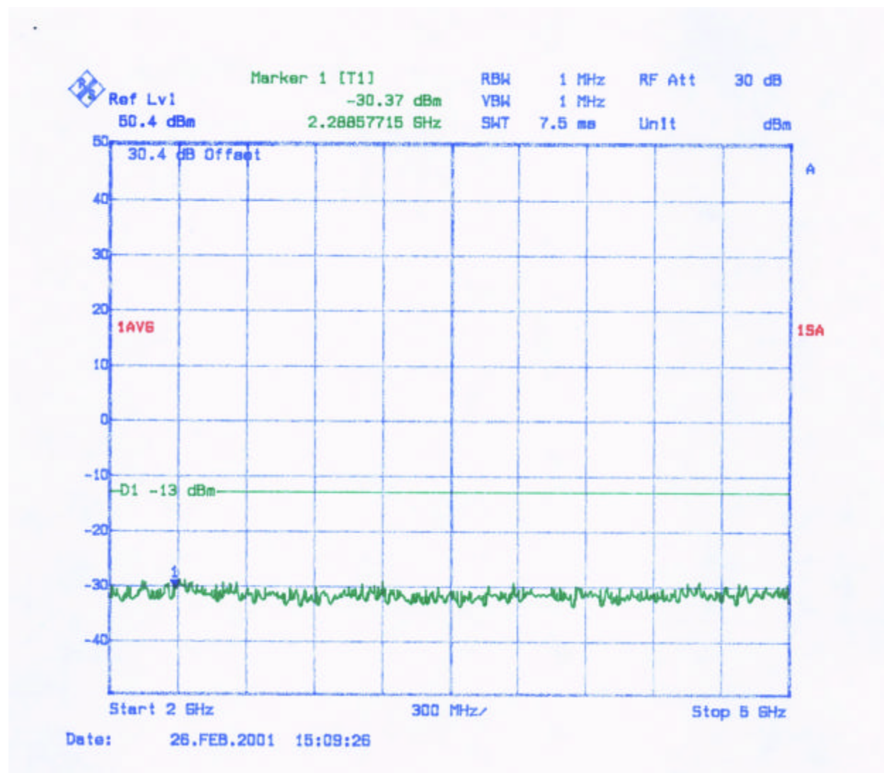
Figure 10: Spurious Emissions – 2 Carrier (2 GHz to 5 GHz)
