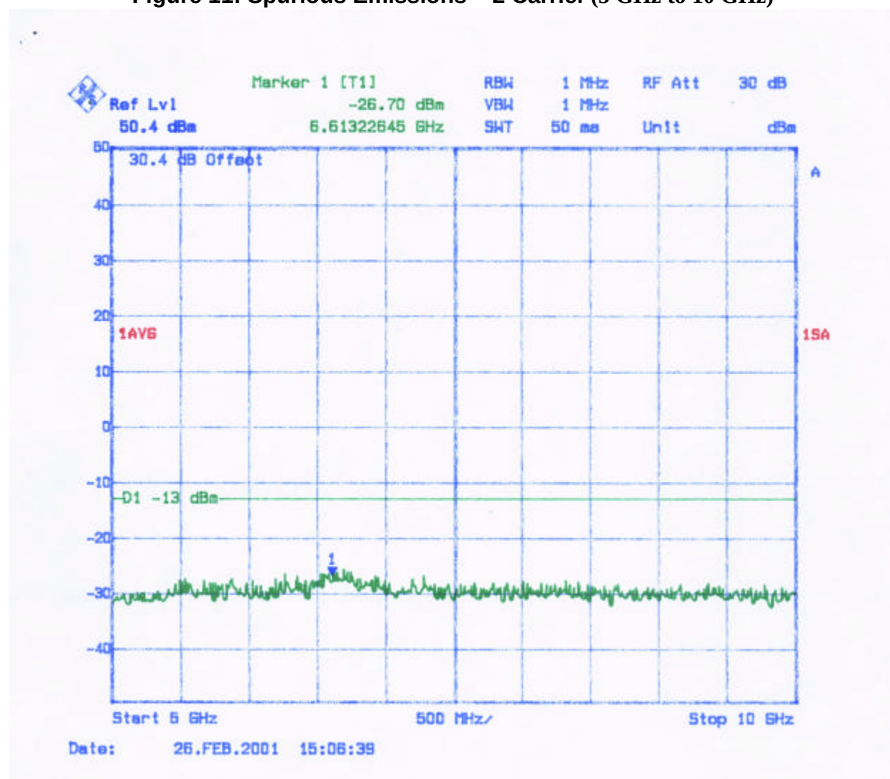
Figure 11: Spurious Emissions – 2 Carrier (5 GHz to 10 GHz)
