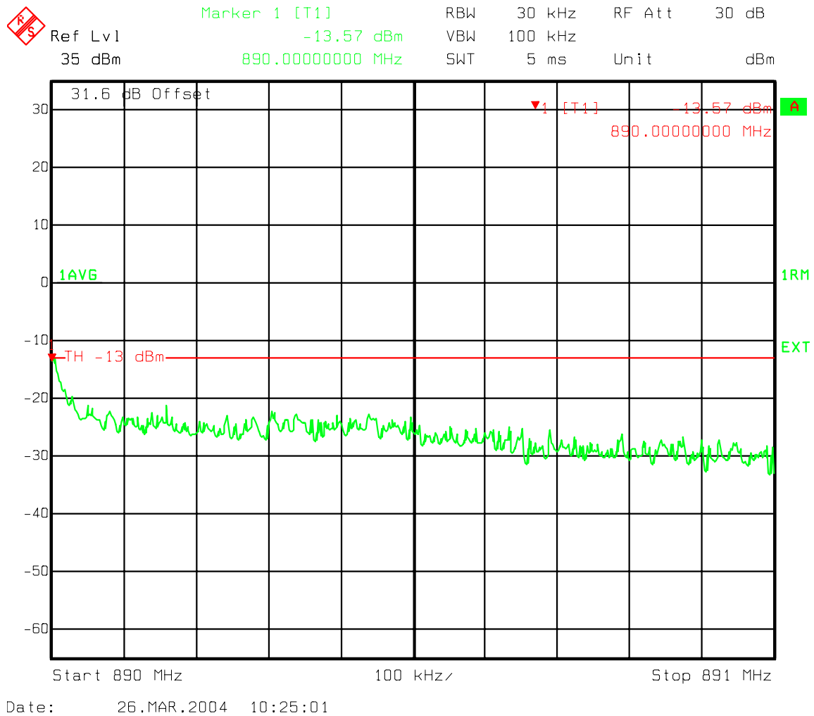
Figure 75 : One Carrier - Ch 642 Upper A Band adjacent 1MHz band emissions
