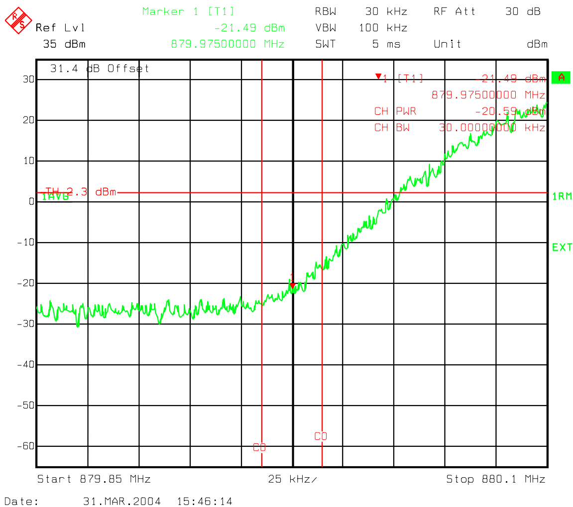
Figure 77 : One Carrier - Industry Canada Lower 750 kHz offset 30 kHz Chan Power Ch 358
