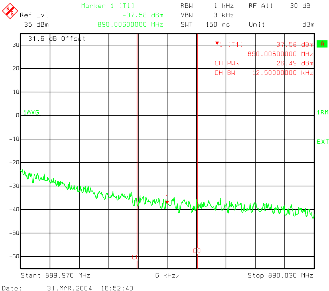
Figure 76 : One Carrier - Ch 642 Upper B Band adjacent to outside edge 12.5 kHz band Channel power
