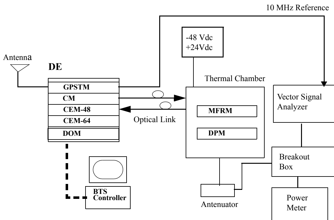
Figure 5 : Test configuration for Frequency Stability
