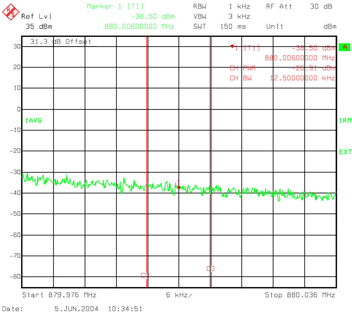
Figure 10 : One Carrier - Ch 308 Upper A Band adjacent to outside edge 12.5 kHz band Channel power
