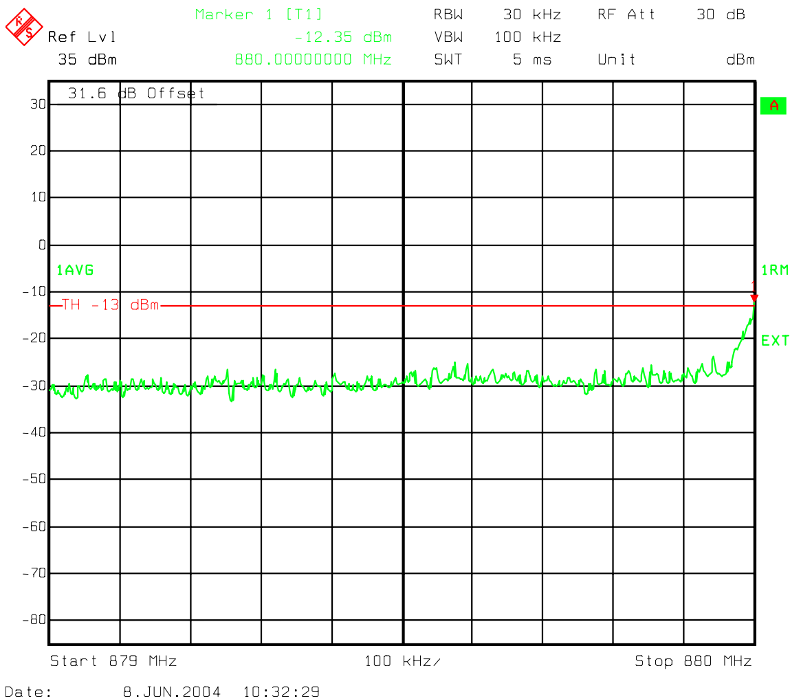
Figure 73 : One Carrier - B Band Ch 358 IS856 Adjacent 1 MHz Lower emissions 879-880 MHz
