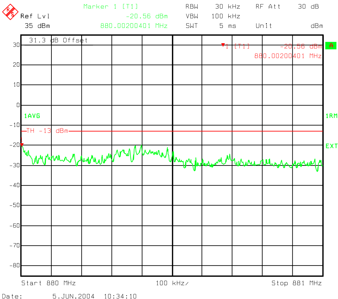
Figure 9 : One Carrier - Ch 308 Upper A Band adjacent 1MHz band emissions
