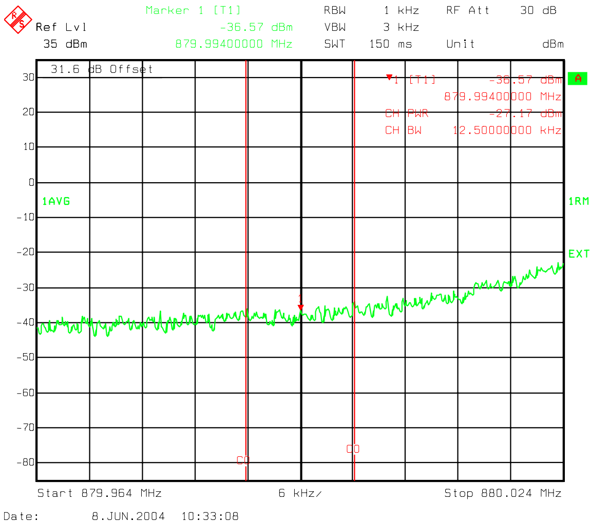
Figure 74 : One Carrier - Ch3585 IS856 Lower B Band Adjacent to outside edge 12.5kHz band Channel Power
