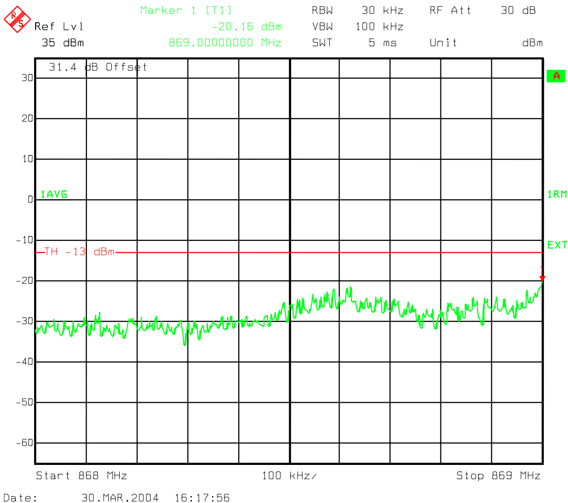
Figure 7 : One Carrier - A '' Band Ch 1015 IS95 Adjacent 1 MHz Lower emissions 868-869 MHz
