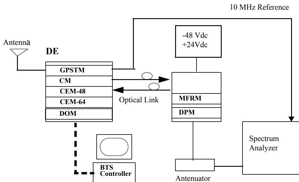
Figure 2 : Test Setup for Occupied Bandwidth Measurement
