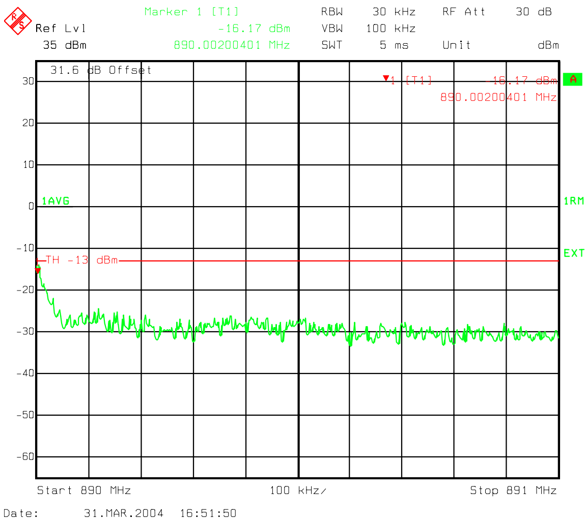
Figure 75 : One Carrier - Ch 642 Upper A Band adjacent 1MHz band emissions
