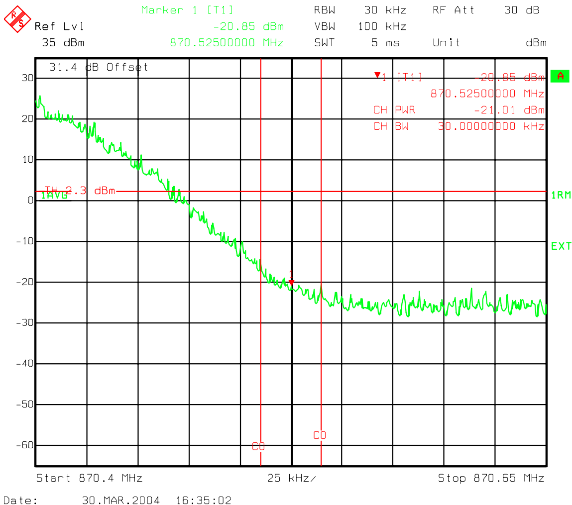
Figure 12 : One Carrier - Industry Canada Upper 750 kHz offset 30 kHz Chan Power Ch 1015
