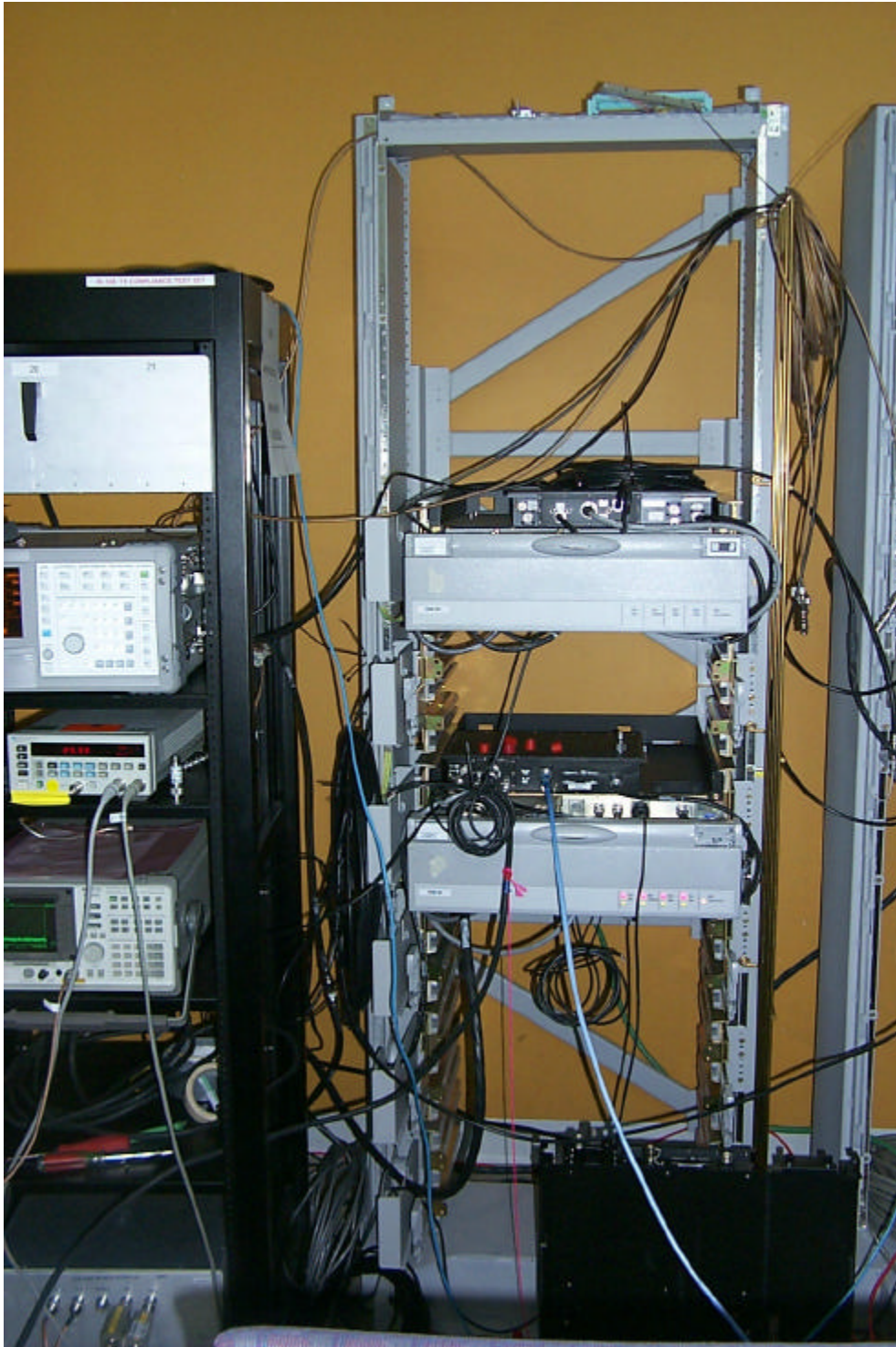
RADIO TEST SETUP PICTURE 1 : MFRM RADIO 800 MHz SYSTEM
