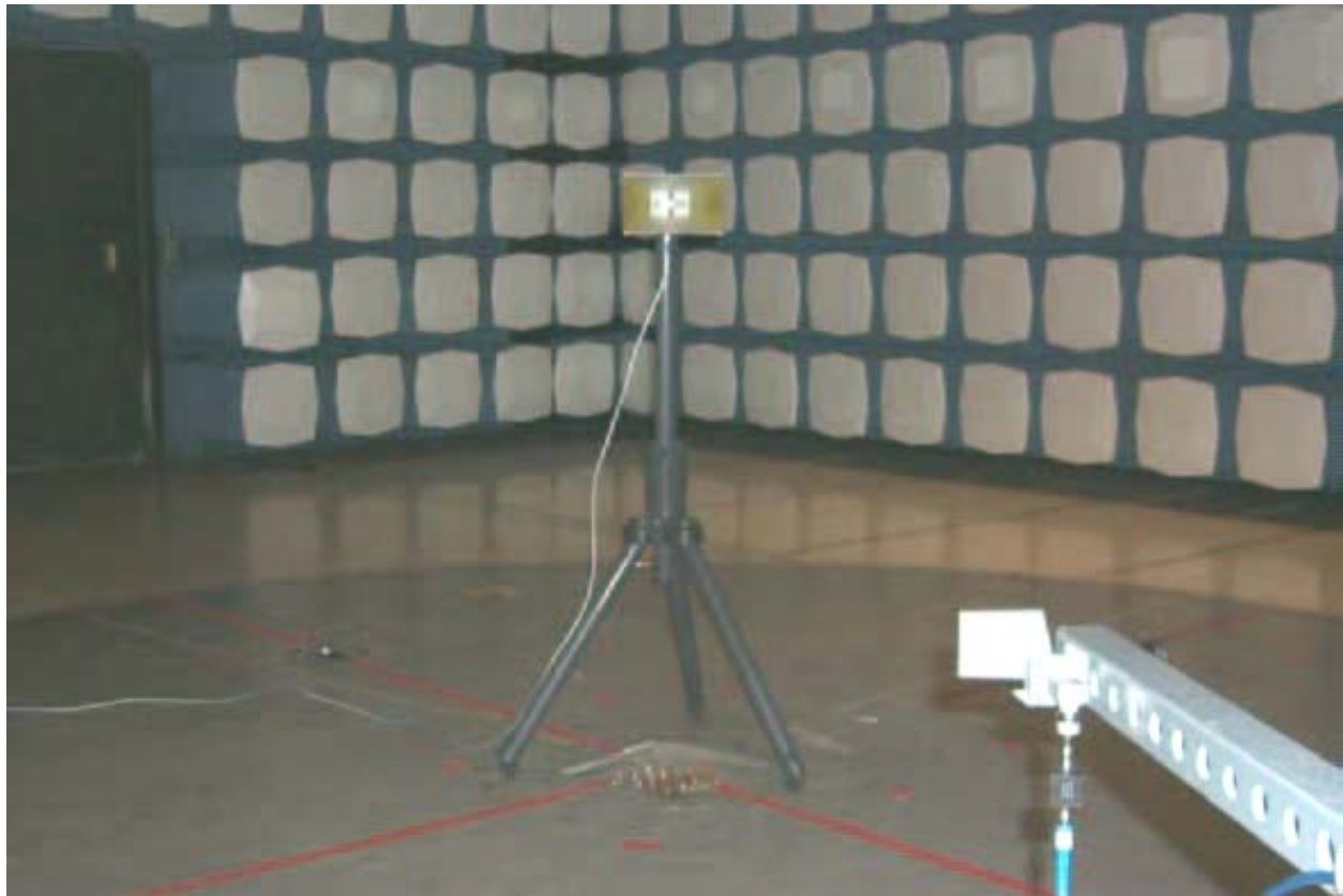
Test setup for the Radiated Emission Signal Substitution Measurement Setup
