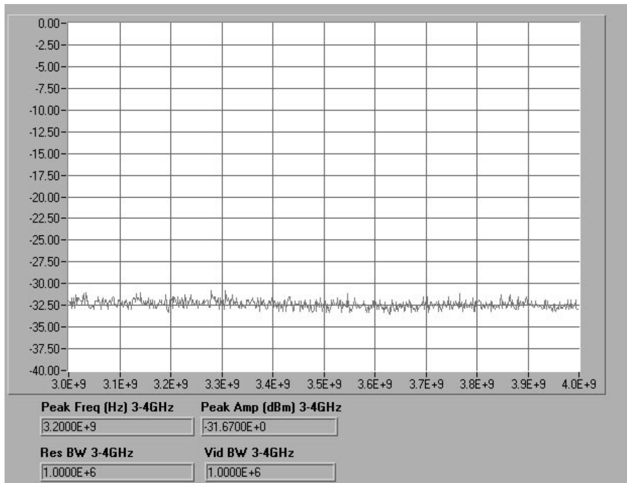
Figure 10 : Conducted Spurious Emissions - Channel 616 (B) 3-4GHz
