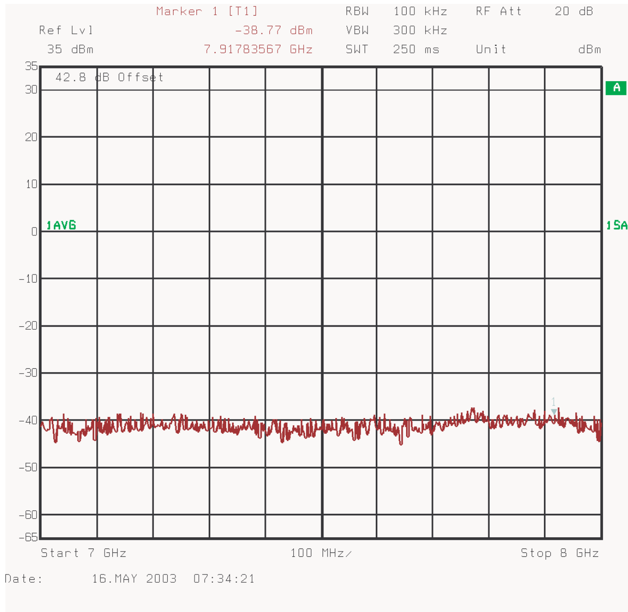
Figure 14 : Conducted Spurious Emissions - 1 Carrier, Channel 17 (7 GHz - 8 GHz)
