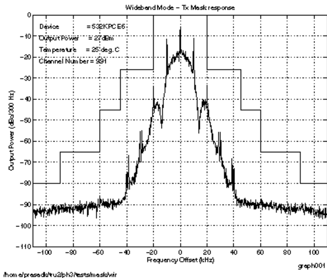
Figure 9: Occupied Bandwidth (Analog) with Wideband Data on Channel 991
