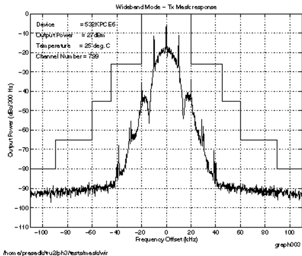
Figure 11: Occupied Bandwidth (Analog) with Wideband Data on Channel 799
