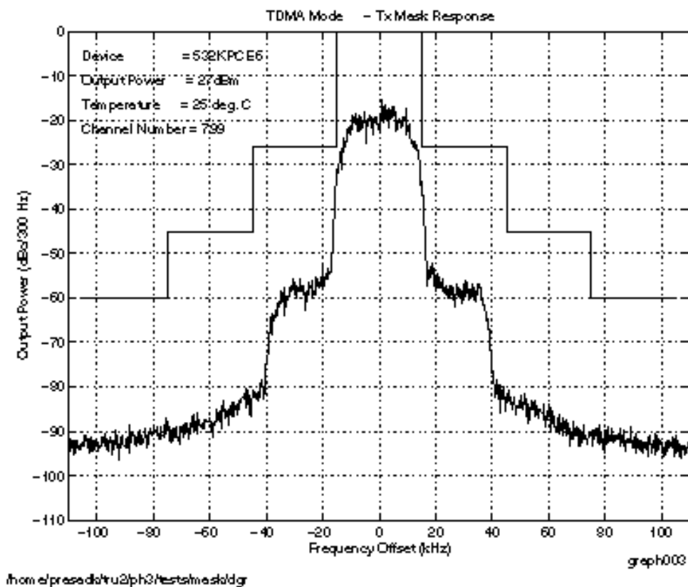
Figure 5: Adjacent Channel Power for Channel 799 (Digital)
