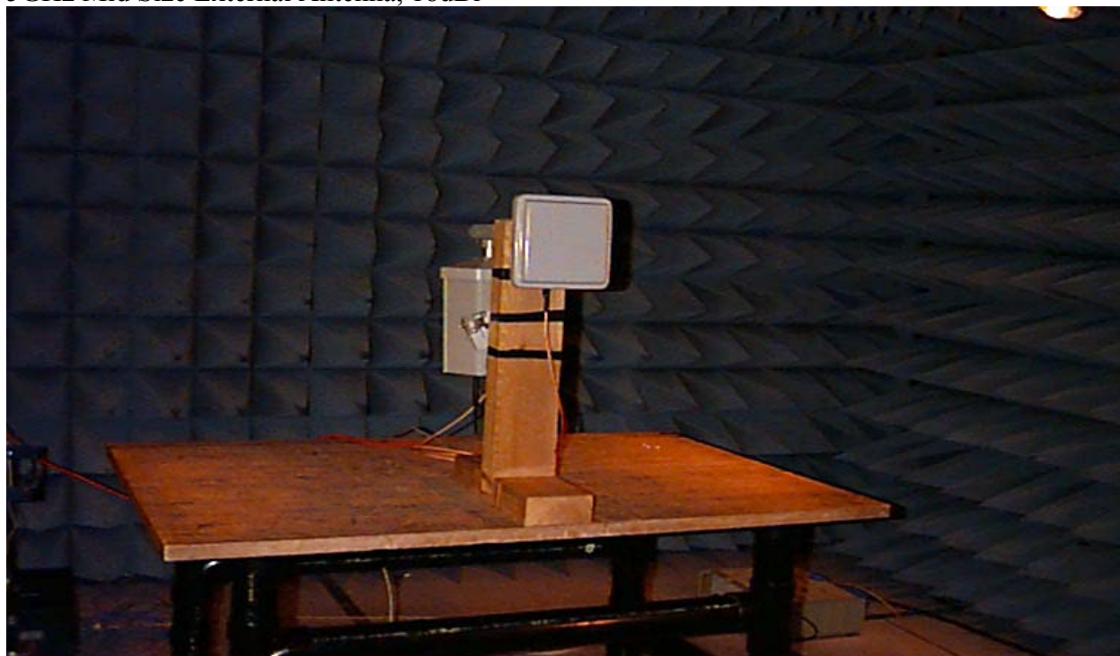
5GHz Mid Size External Antenna, 18dBi
