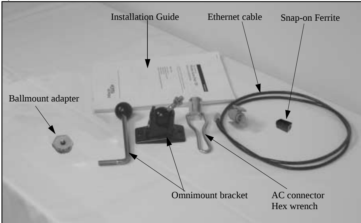
Figure 1-3 Optional accessories
