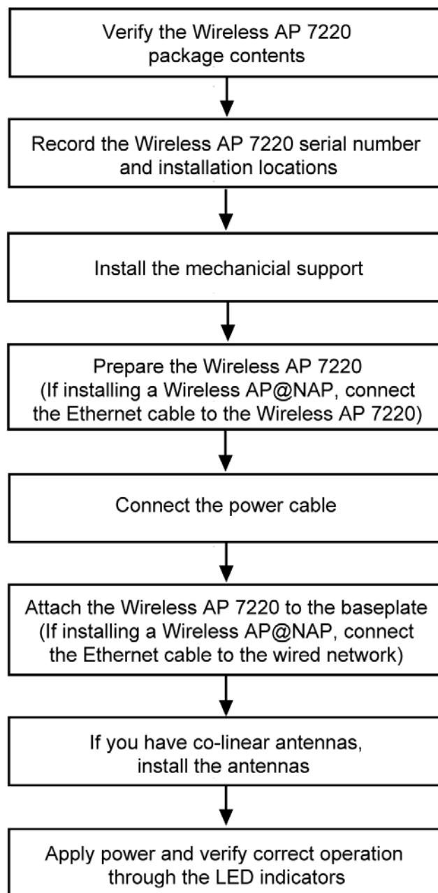
Figure 1 Installing the Wireless AP 7220 flowchart
