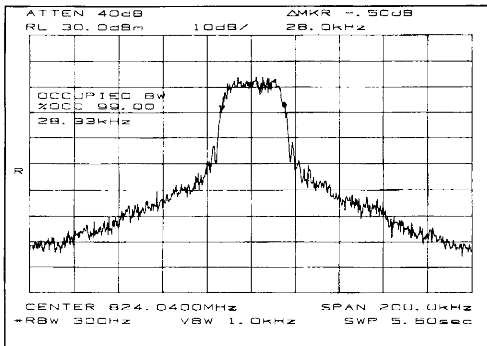
Figure 1: 99% Occupied Bandwidth (Channel 991)
