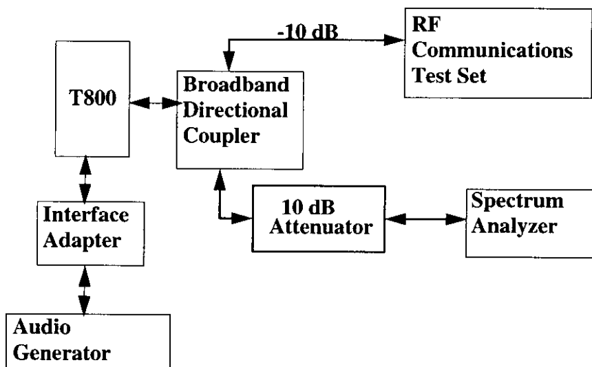
Test setup to measure emissions from 100 kHz to 10 GHz
