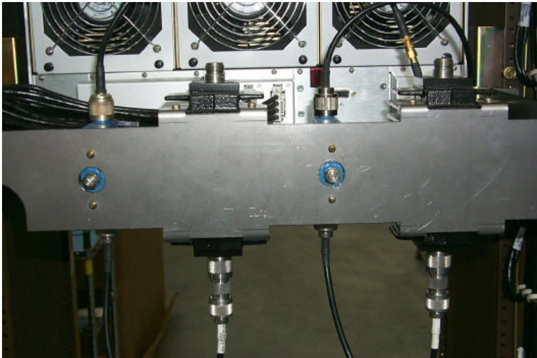
Figure 4: Detailed Rear View of the Adjunct Kit
