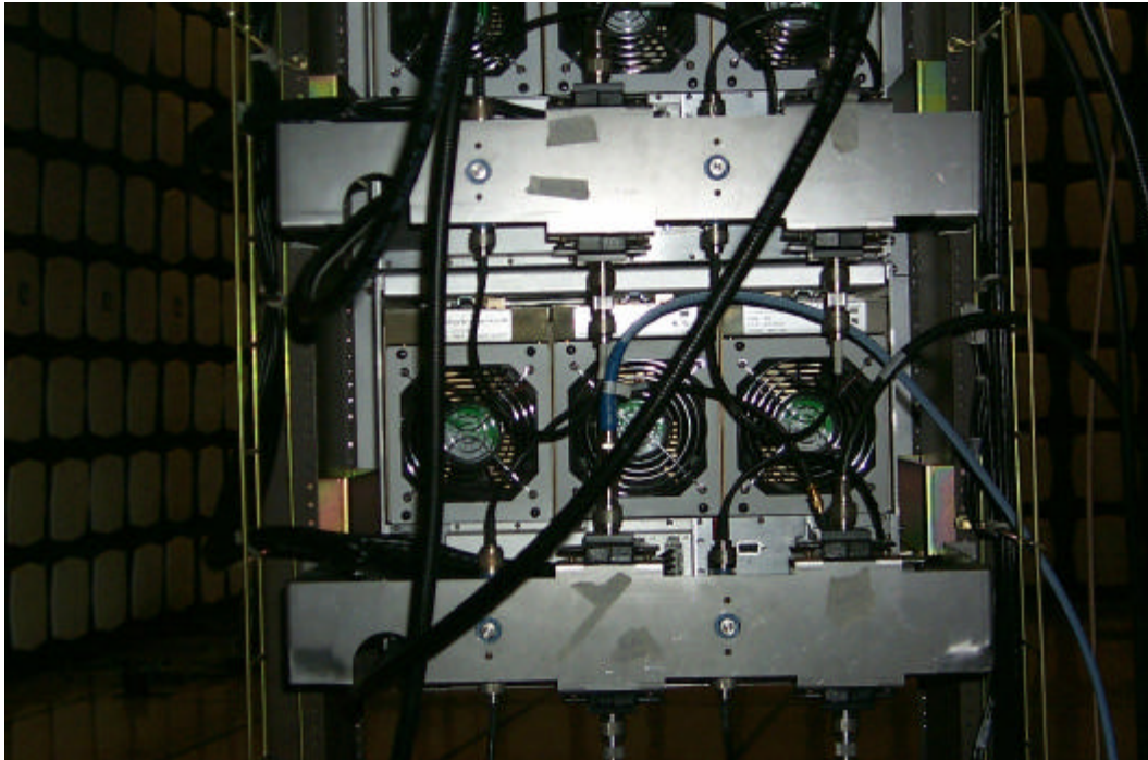
Figure 3: Rear View of the MCPA Shelf with Adjunct Kit
