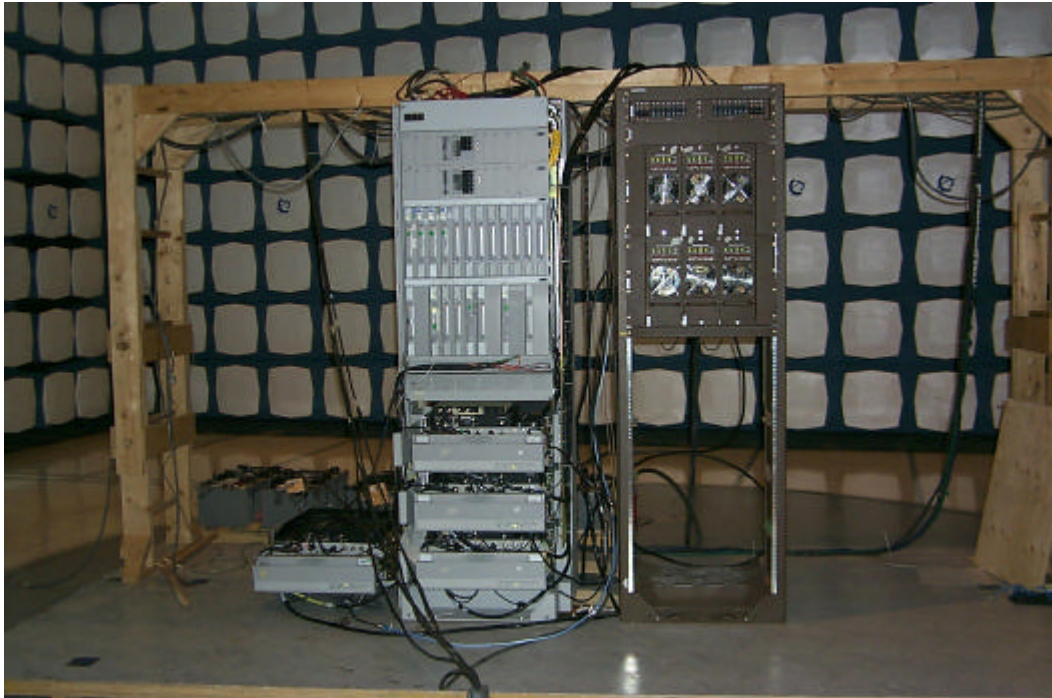
Figure 1: Front View of CDMA Digital Rack and TDMA RF Rack
