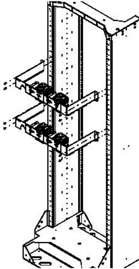
Figure 10: Frame Assembly
