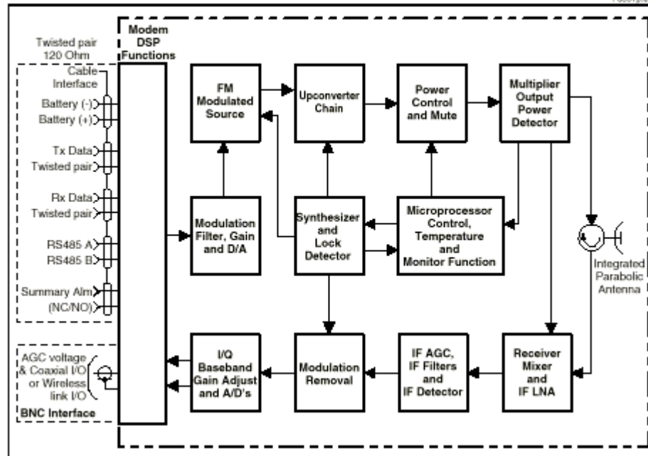
Figure 1-2 Internet BWA System 3200 components—block diagram
