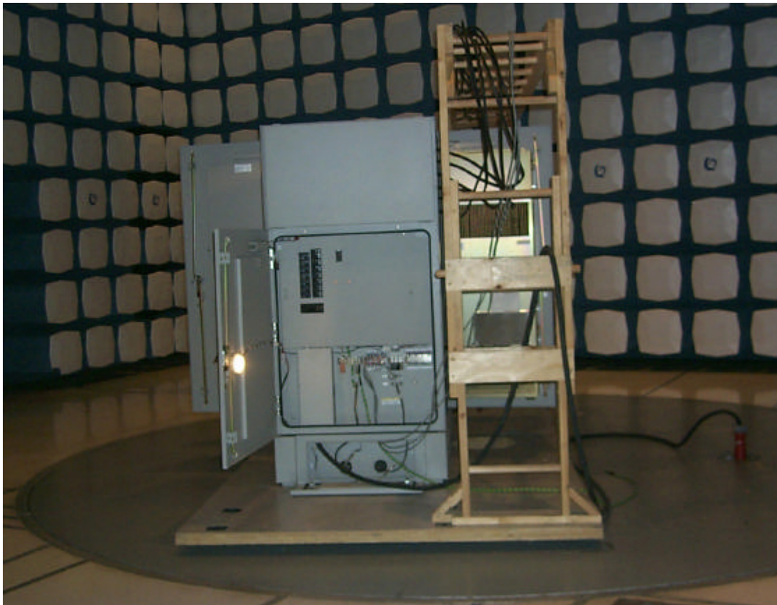
Figure 5: Door Open Side View of the TDMA 800MHz Enclosure System
