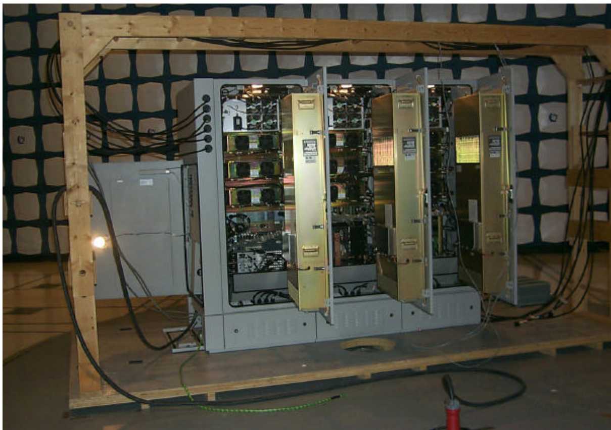
Figure 4: Doors Open Rear View of TDMA 800MHz Enclosure System
