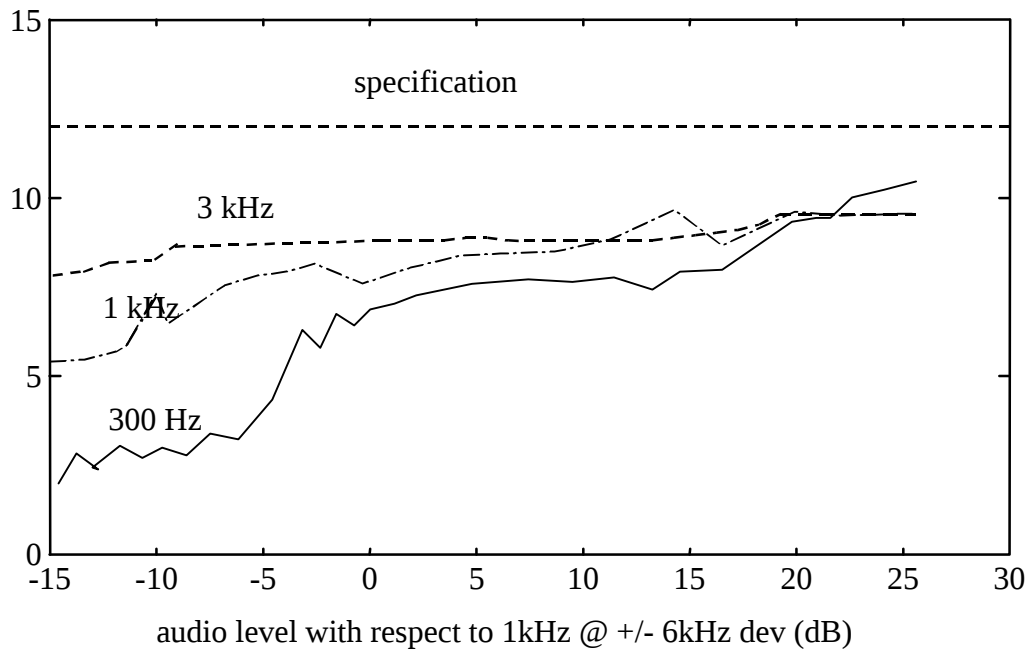
Figure 4.4.1: Deviation Limiting
