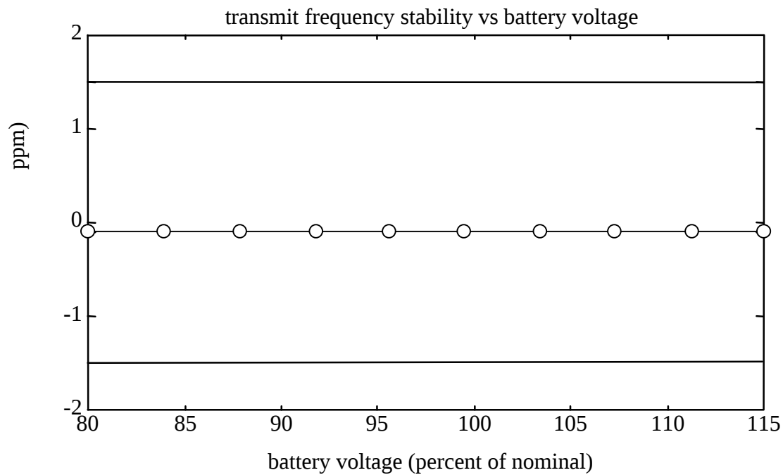
Figure 4.7b: Frequency Stability versus Battery Voltage
