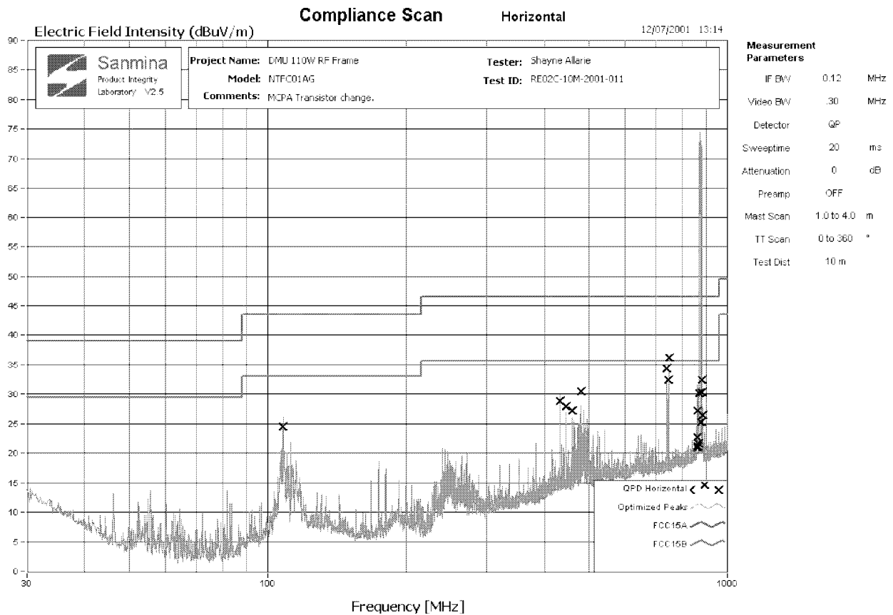
Figure B1 – Radiated Emissions 30 MHz to 1GHz H-Pol
