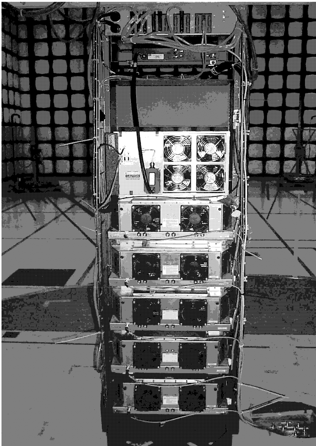
Figure C5 – EUT Rear View
