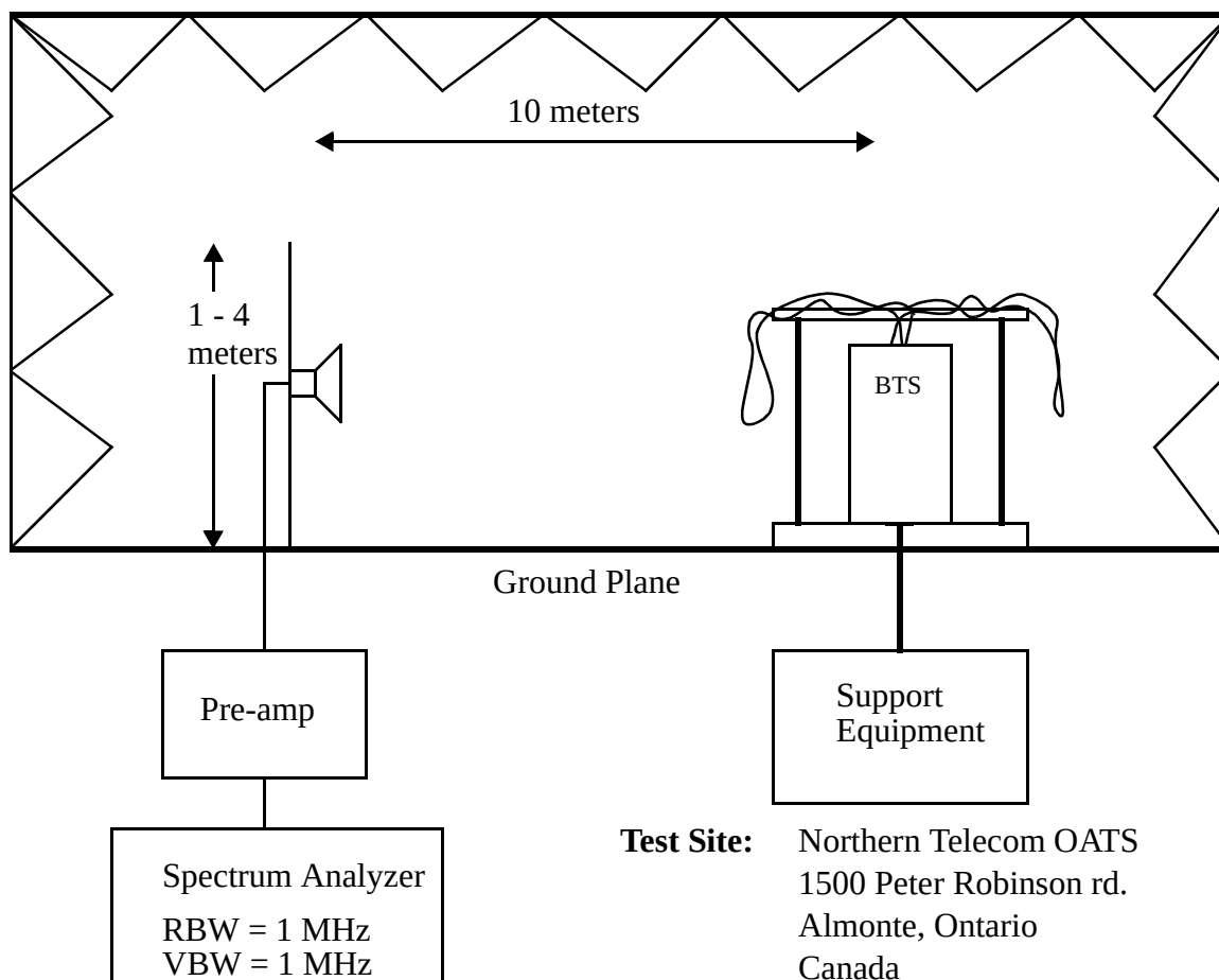
Figure 6: Test Configuration for Radiated Spurious Emissions
