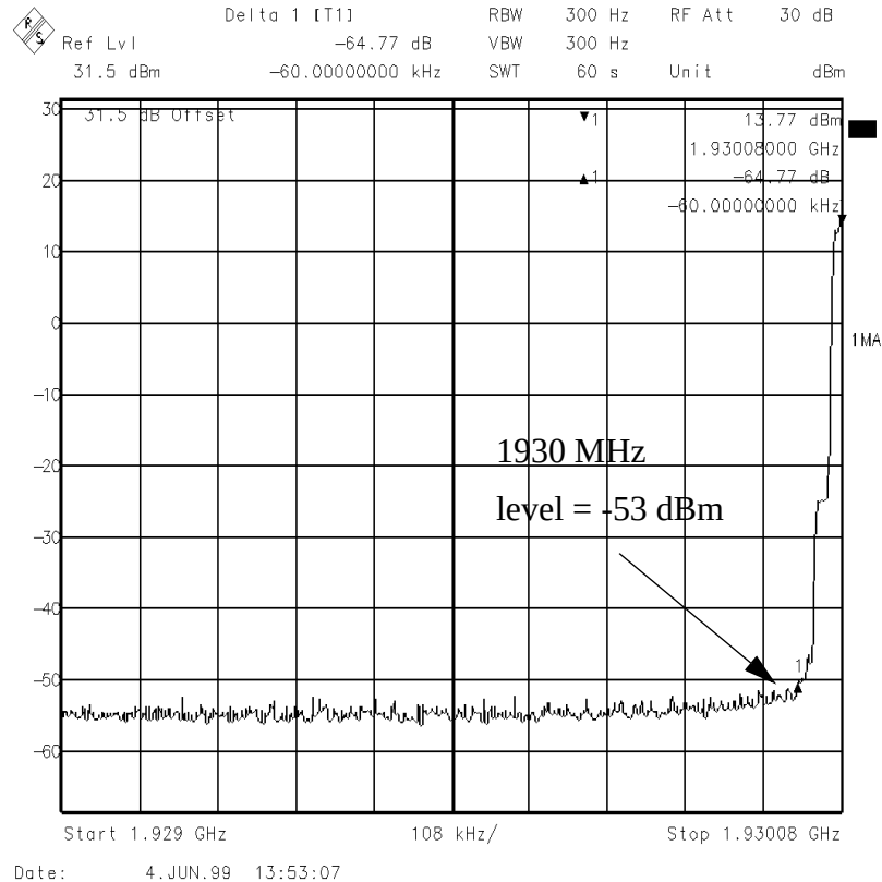
Figure 4: Sample Plot for Ch. 2 (1st Adjacent MHz)
