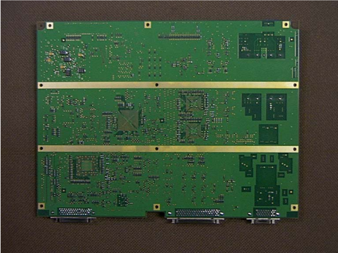
Figure 2 – E-LDRX (Logic Board) Bottom View
