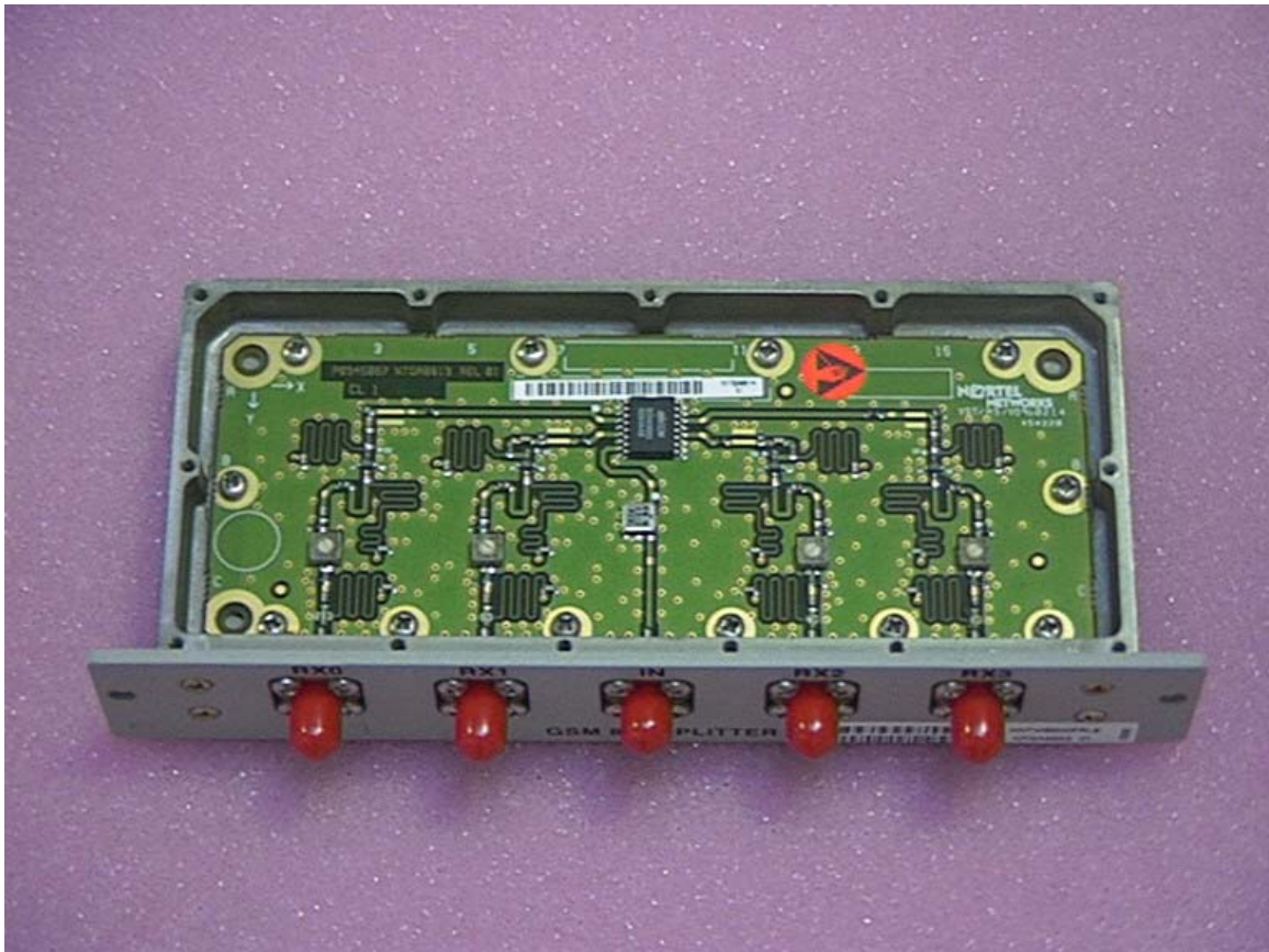
Figure 6 – RX Splitter Bottom View
