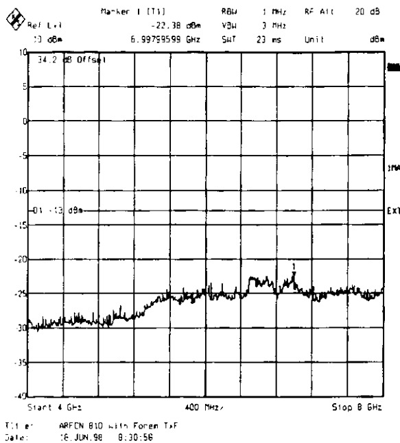
Figure 10 : Out of block emissions (Channel 810, Pmax - 12 dB)
