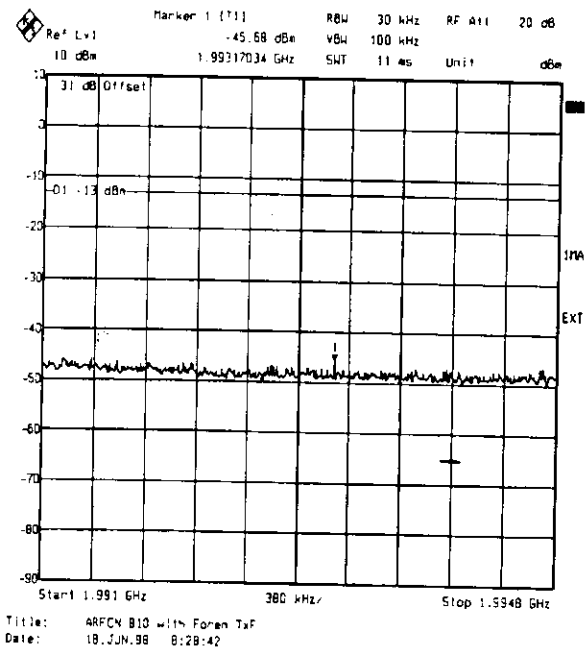
Figure 9 : Out of block emissions (Channel 810, Pmax - 12 dB)
