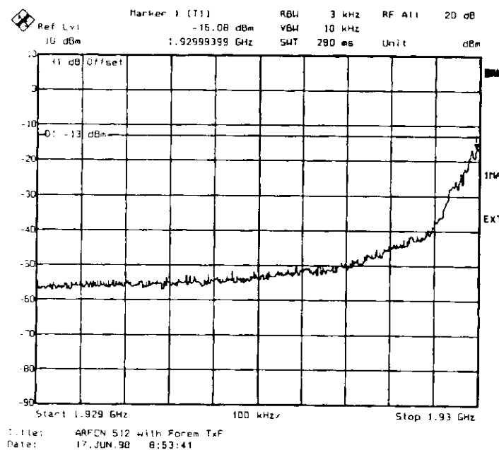
Figure 3 : -1 MHz adjacent band (Channel 512, Pmax - 12 dB)
