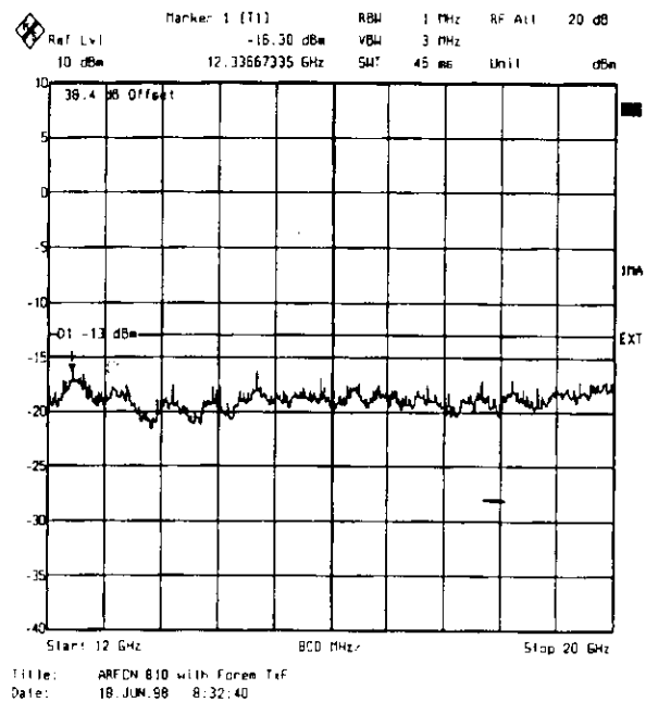
Figure 10 : Out of block emissions (Channel 810, Pmax - 12 dB)
